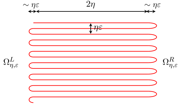
Figure 1: The oscillatory interface \Gamma_{\eta,\varepsilon} separates \Omega_{\eta,\varepsilon}^L and \Omega_{\eta,\varepsilon}^R . It has two scales: its amplitude \eta and period \eta\varepsilon
