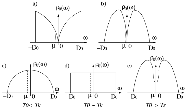
FIG. 1. Schematic non interacting DOS: singular (a and b), semi-elliptic (c), constant (d), and pseudo-gaped (e). As soon as \rho_0(\omega = \mu) \neq 0 , the Kondo temperature T_K is finite. Close to the half-filling, the shape of the DOS around \mu is crucial for determining the Fermi-liquid temperature: (c) \mu is close to a maximum of \rho_0 and T^* < T_K . (e) \mu is close to a minimum of \rho_0 , and T^* > T_K . (d) \rho_0 is constant and T^* \sim T_K .
