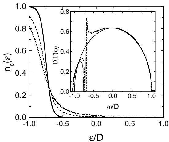
FIG. 4. n_c(\epsilon) for T/T_K=1.0 (solid line), 0.5 (dashed line), 0.005 (dotted line). n_c=0.15 . Inset: Spectral density \Gamma(\omega) for T/T_K=1 (solid line), 0.5 (dashed line) and 0.25 (dotted line). For T < T_K there is a \delta -function peak in the gap not shown for clarity. n_c=0.2 . In all plots J_K/D=0.75 .
