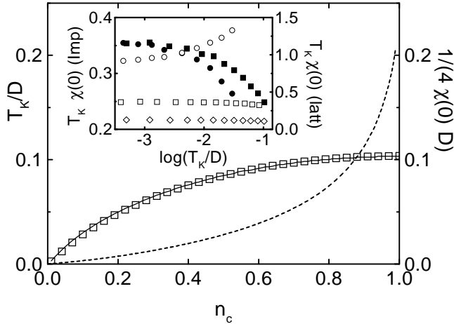
FIG. 1. Solid line: density-dependence of T_K (defined as the slave boson condensation temperature). Squares: 1/4\chi_f(T=0) for a single impurity. Dashed line: 1/4\chi_f(T=0) for the lattice. J_K/D=0.75 . Inset: T_K\chi_f(0) for the impurity (left scale, solid symbols) and the lattice (right scale, open symbols) for n_c=0.1, 1.0 (impurity) and n_c=0.1, 0.5, 0.9 (lattice) from top to bottom. All plots are for a semi-circular d.o.s.
