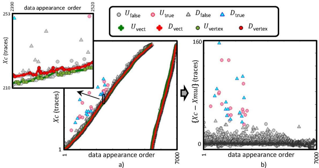
Figure 3. Proposed change of the space by X_c property. a) X_c , and b) \{X_c - X_{\text{mul}}\} .
