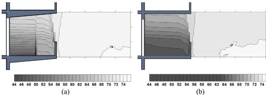
Fig. 11. Balcony cross section shows the maximum effect of the inclined ceiling, for a balcony with 3 m depth, and with an angle equal to 5^\circ (a), and the classical ceiling form (b) at the 11th floor.
