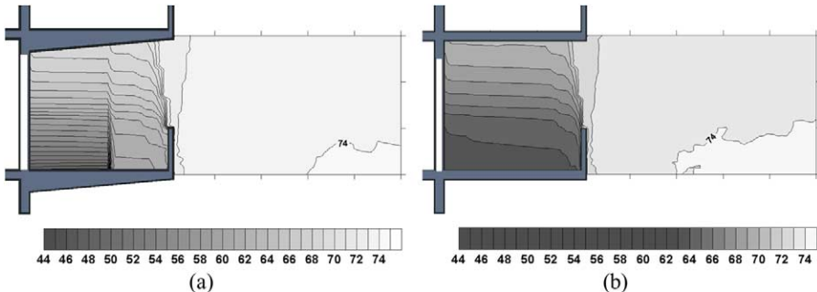
Fig. 11. Balcony cross section shows the maximum effect of the inclined ceiling, for a balcony with 3 m depth, and with an angle equal to 5^\circ (a), and the classical ceiling form (b) at the 11th floor.
