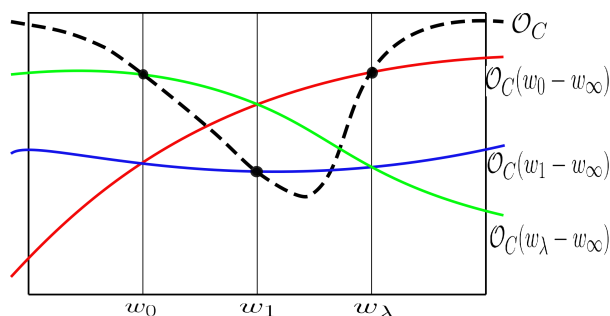
FIGURE 3. Sections of \mathbb{P}E_1
