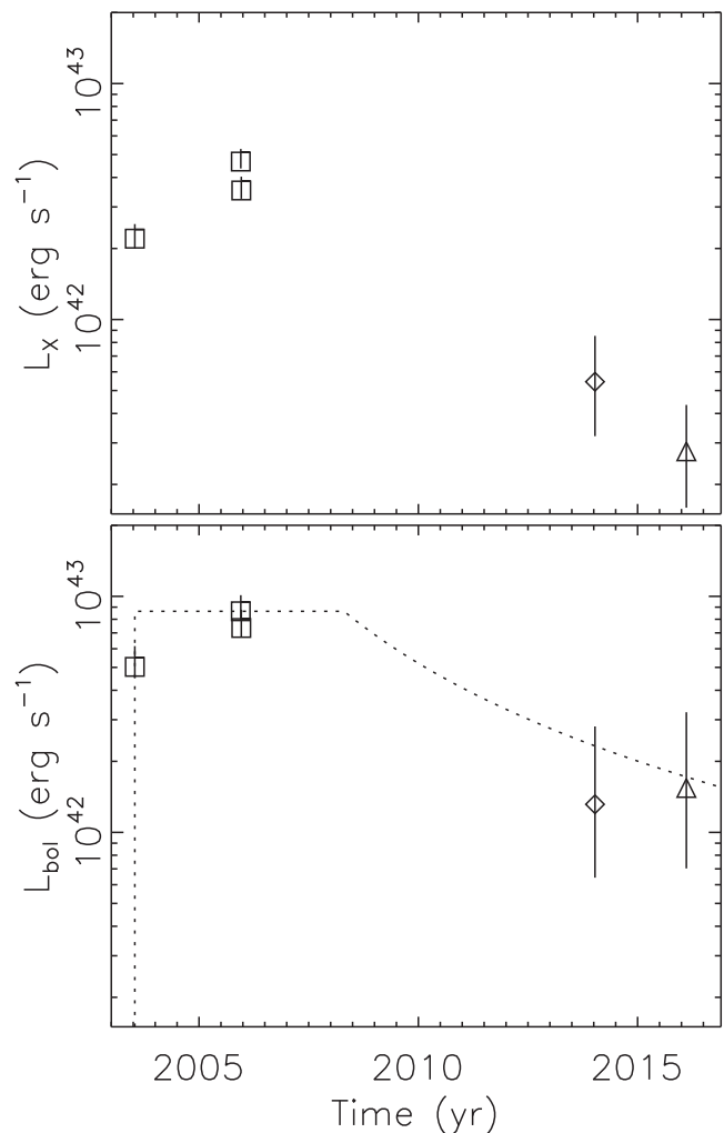
Figure 5. The long-term luminosity curve of XJ1231+1106 from the XMM-Newton (squares), Swift (diamond), Chandra (triangle) observations. The upper panel is for the 0.34–11 keV (source rest frame) unabsorbed luminosity, and the bottom panel is for the bolometric luminosity based on the MCD model. The dashed line plots a TDE model of prompt accretion (see Section 4 for more details).
