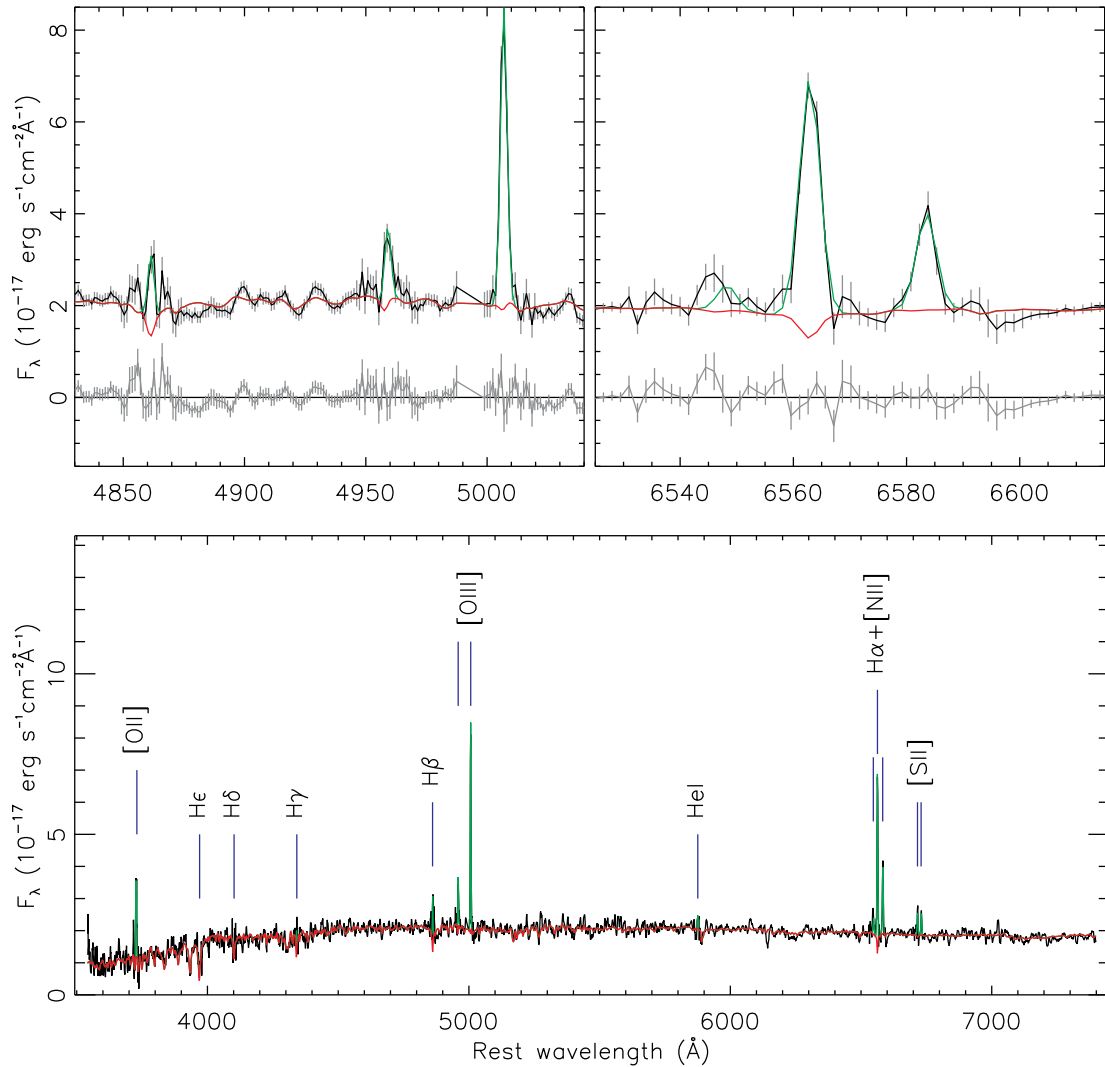
Figure 1. The SDSS optical spectrum of the candidate host galaxy of XJ1231+1106 taken on 2012 March 3, showing only narrow emission lines. The upper two panels zoom into the H \beta -[O III] complex and the H \alpha -[N II] region, with the fit residuals. The PPF fit is shown as a solid green line, while the star component is shown as a red line. The data points outside the emission line regions have been smoothed with a box function of width 5 for clarity.
