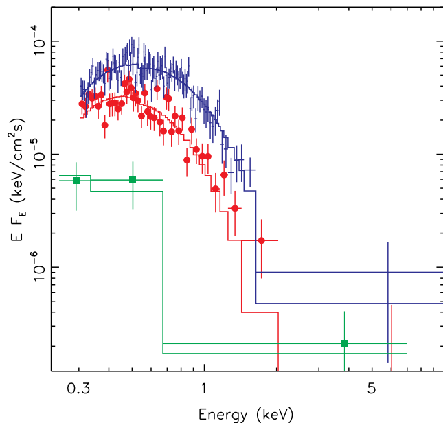
Figure 4. The example unfolded spectra of XJ1231+1106 fitted with the MCD model. From the top to the bottom are the second XMM-Newton observation (blue), the first XMM-Newton observation (2003 July 13, red filled circles) and the Chandra observation (green filled squares). For clarity, we show the pn data only for the XMM-Newton observations and have rebinned all spectra to be above 2\sigma per bin.
