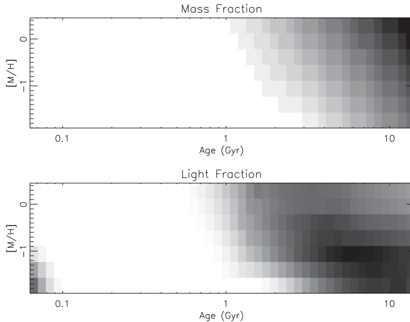
Figure 2. Relative mass and light fractions of different stellar populations in the host galaxy of XJ1231+1106 with respect to metallicity and age, with darker shading indicating a larger mass fraction in the best-fitting model. There seems to be a young (<90 Myr) population, based on the light fraction plot. The light was integrated over 3540 and 7410 Å.
