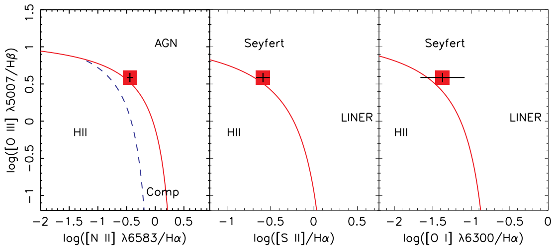
Figure 3. XJ1231+1106 on the BPT diagrams, indicating it as an AGN possibly with some star-forming activity. The dashed and solid lines are used to separate galaxies into H II-region-like, AGN and composite types (Kewley et al. 2006).
