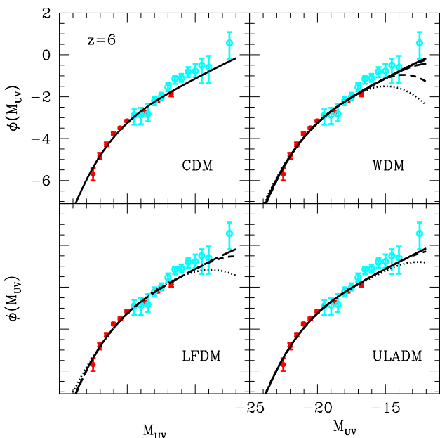
FIG. 14: As in Fig. 11 for L16 data at z = 6 (cyan filled circles).
