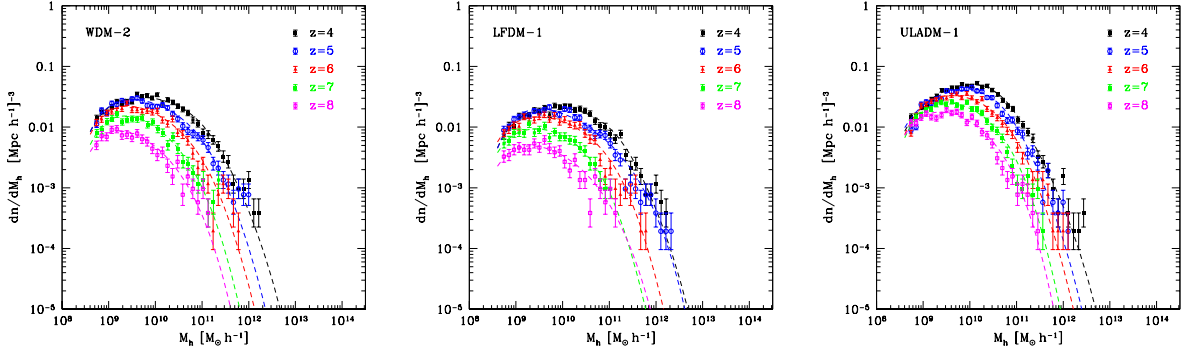
FIG. 15: Halo mass function from N-body halo catalogs of WDM-2 (left panel), LFDm-1 (center panel) and ULADM-1 (right panel) and best-fit functions at z = 4, 5, 6, 7 and 8 (data points and curves from top to bottom)
