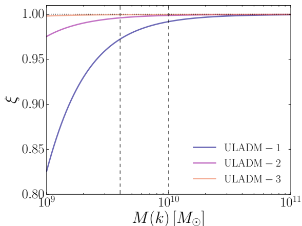
FIG. 3: The growth rate ratio, \xi , defined in [82] for the ULADM models for z_{\text{start}} = 100 and z_{\text{end}} = 4 as function of the mass scale M(k) = 4\pi(\pi/k)^3 \rho_m/3 , where \rho_m is the comoving matter density. The vertical dotted lines denotes the lowest mass scales probed by HST observations of the faintest galaxies at 4 \lesssim z \lesssim 8 . Unlike [82], our initial conditions use the correctly evolved initial conditions from AXIONCAMB; we use \xi as a measure of the importance of scale-dependent growth to assess how well ULAs can be modelled with N -body simulations. The lightest ULA model we consider is well described by collisionless simulations at the percent level for halo masses of interest.
