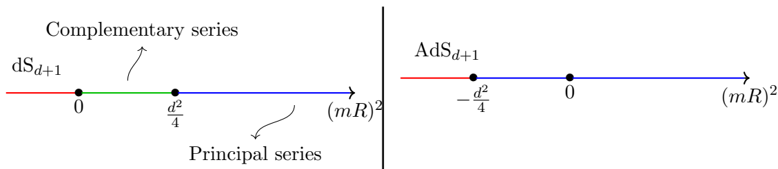
Figure 1. Unitary (blue and green), and non-unitary (red) regions for the squared mass of a scalar field in de Sitter (left) and anti-de Sitter space (right).
