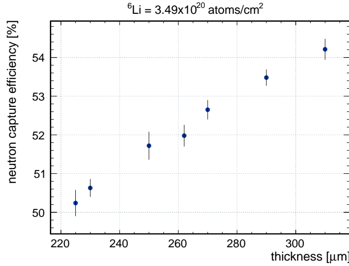
Figure 5. Simulated neutron capture efficiency as a function of the screen thickness for a fixed {}^6\text{Li} concentration of 3.49 \times 10^{20} \text{ atoms/cm}^2 .
