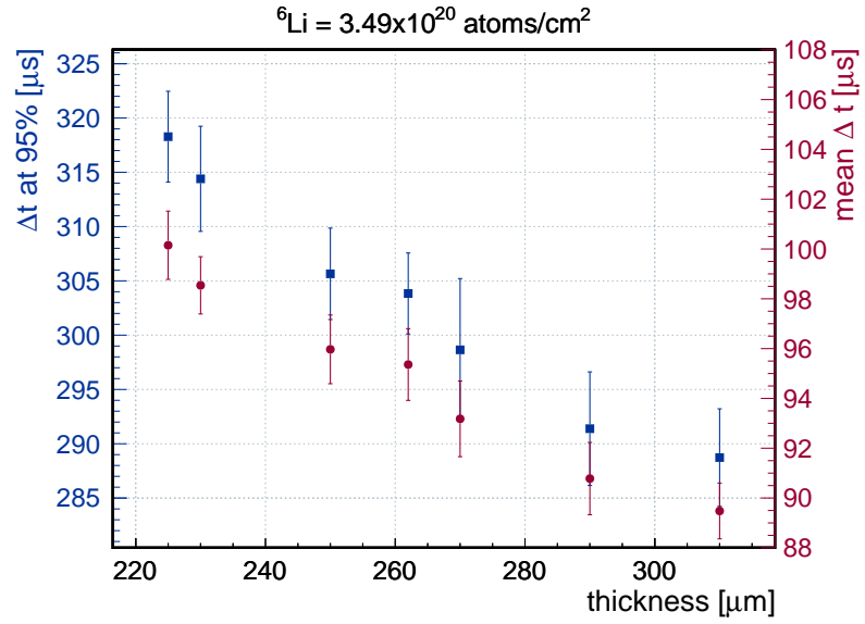
Figure 6. Simulated neutron capture time as a function of the screen thickness for a fixed {}^6\text{Li} concentration of 3.49 \times 10^{20} atoms/cm 2 . The capture time can be expressed as the mean of the distribution of capture times (red) and as the value below which 95% of all the capture times are contained (blue).
