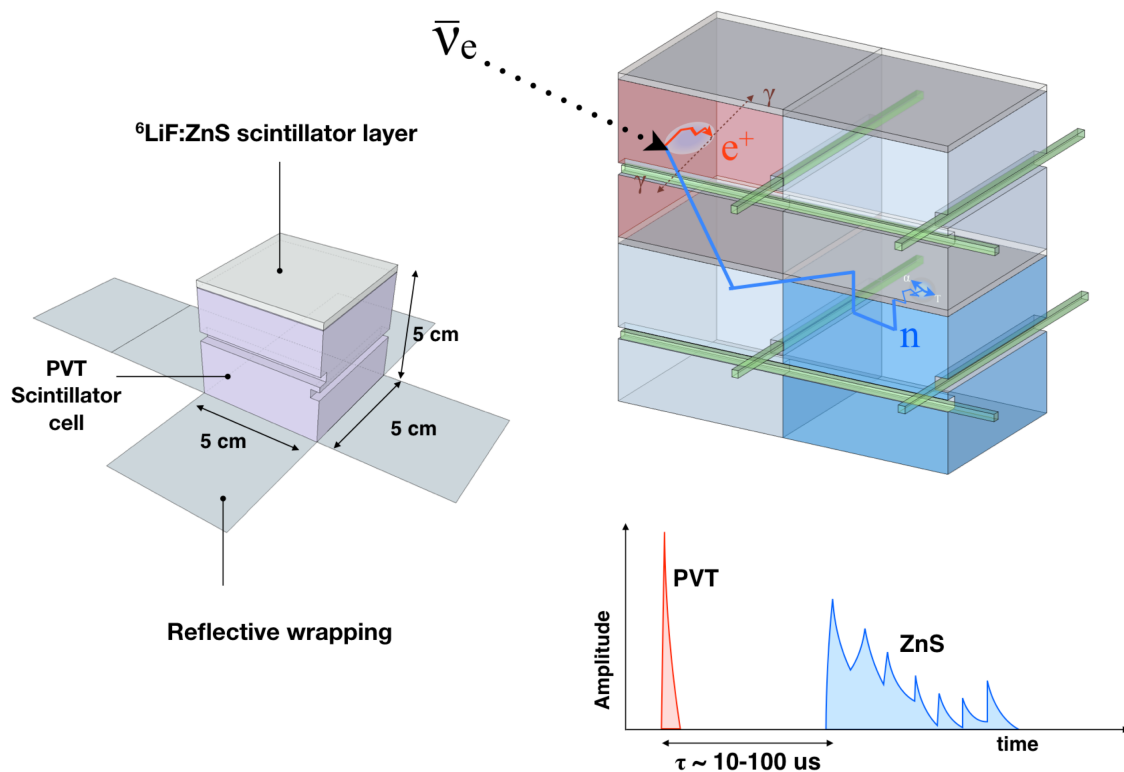
Figure 1. (Left) The PVT cube is covered with a layer of {}^6\text{LiF:ZnS}(\text{Ag}) and the assembly wrapped in a reflective material. (Top right) Principle of \bar{\nu}_e detection in a volume made of separated voxels: wavelength shifting fibres placed in perpendicular orientations are used to collect the scintillation light from each cell of the array. (Bottom right) Time spectrum of PVT and ZnS(Ag) scintillation, used to identify the IBD reaction products.
