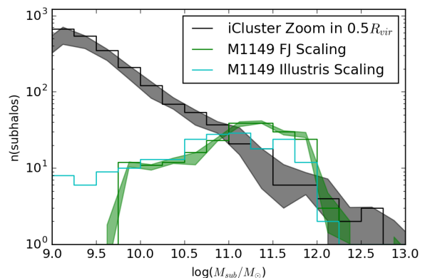
Figure 21. Comparing lensing derived SHMFs for different assumptions relating mass to light: here we plot the SHMFs (with model errors) derived from the best-fit lensing model for MACSJ 1149 using the Faber-Jackson and Kormendy luminosity scaling laws, with that derived for the best-fit lens model using the scaling laws from the full physics run of iCluster Zoom 1 .
