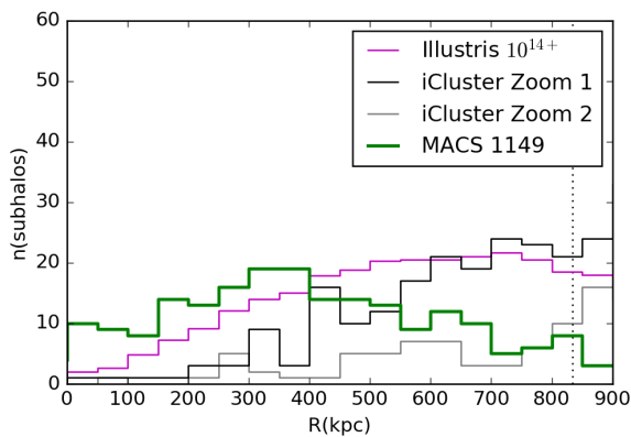
Figure 26. Radial distribution of the sub halo mass function derived from simulated Illustris clusters and iCluster Zoom 1 compared to that of the lensing derived SHMF for MACSJ 1149 from the HST FF data (green histogram). Once again the most massive 66 simulated clusters with M > 10^{14+} M_{\odot} were selected at z = 0.45 - 0.65 from the Illustris simulation box comprising the 10^{14} Illustris Haloes were selected from the full physics run of Illustris. We also plot the radial distribution of the count matched sub haloes from two iCluster Zooms . We clearly see in this case that surprisingly, galaxies in the simulations do better mimic the distribution in MACSJ 1149 in the inner regions than for the other two HSTFF cluster lenses.
