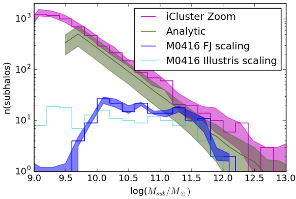
Figure 14. Comparison with the analytically predicted SHMF: the lensing derived SHMF (with model errors) for the two independent scaling laws is over-plotted along with the analytically calculated SHMF for a cluster halo with mass equivalent to that of MACSJ 0416. This analytic estimate includes the halo-to-halo scatter that is shown in the dull green band.
