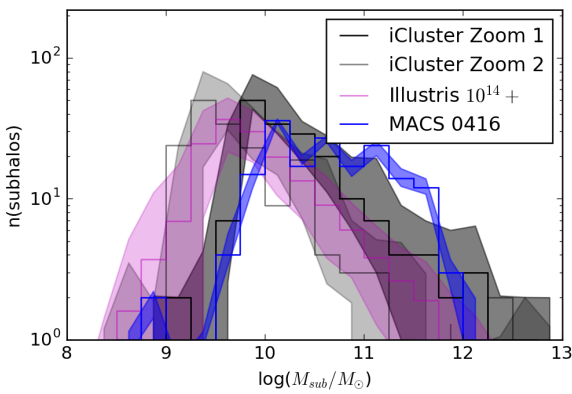
Figure 15. Comparison of the SHMF derived for MACSJ 0416 from the HST FF data (blue histogram) with that derived from the two massive zoomed-in simulated clusters iCluster Zooms (the z \sim 0.4 full physics run snapshots) and the 10^{14} Illustris Haloes of M > 10^{14+} M_{\odot} mimicking the observational selection in all of them. Here only subhaloes that host the brightest 175 cluster galaxies (number matched to the HSTFF data of MACSJ 0416 are included) selected from the simulations. The 1\sigma cluster-to-cluster variations are once again plotted as the bands.
