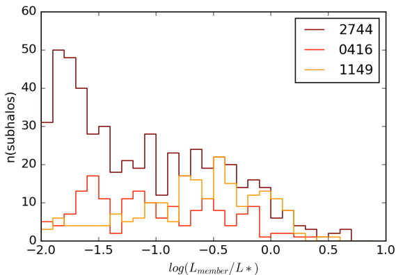
Figure 2. The cluster galaxy luminosity selection for our analysis in Abell 2744, MACSJ 0416 and MACSJ 1149. As seen here clearly, the larger number of identified strong lensing systems and their modeling plus the lower redshift of Abell 2744 allows us to probe more cluster galaxies down to 0.01 L^* ; while the smaller number of strong lensing systems identified in MACSJ 0416 and MACSJ 1149 provide constraints on fewer cluster members down to the same limit luminosity cut. We use the selected number of 563 cluster galaxies in Abell 2744, 175 in MACSJ 0416 and 217 in MACSJ 1149 in all further analysis presented in this work.
