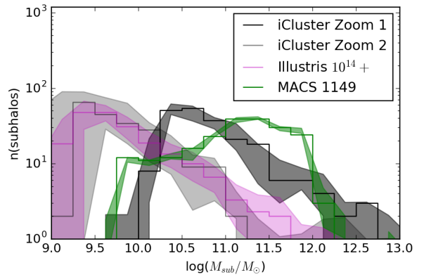
Figure 24. Comparison of the SHMF derived for MACSJ 1149 from the HST FF data (green histogram) with that derived from the two iCluster Zooms as well the larger sample 10^{14+} Illustris Haloes with M > 10^{14+} M_{\odot} clusters now mimicking the observational selection. Here only subhaloes that host the brightest 217 cluster galaxies (number matched to the HSTFF data of MACSJ 1149) are selected from the simulations. The 1\sigma cluster-to-cluster variations are once again plotted as the bands.
