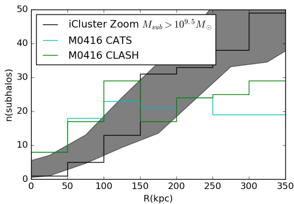
Figure 18. Comparison of sub halo properties in MACSJ 0416 inferred from lens modeling in this work and from the CLASH collaboration (Grillo et al. 2015) with that derived from the 10^{15} M_{\odot} cluster from the Illustris suite - the radial distribution of subhaloes.
