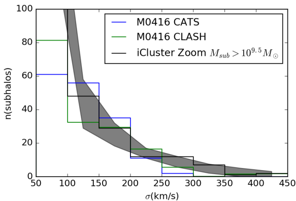
Figure 19. Comparison of sub halo properties in MACSJ 0416 inferred from lens modeling in this work and from the CLASH collaboration (Grillo et al. 2015) with that derived from the 10^{15} M_{\odot} cluster from the Illustris suite - the velocity dispersion function of subhaloes. We find very good agreement between the 2 best-fit mass models and the iCluster Zooms
