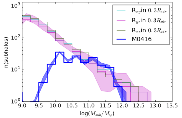
Figure 16. Projection Effects on the derived SHMF: here we plot the SHMF derived from Illustris clusters derived by projecting along several distinct axes within 0.3 R_{\text{vir}} . We note that projection effects cannot account for slight excess seen in the observationally determined SHMF in MACSJ 0416 (blue histogram) and the determinations from iCluster Zoom 1 .
