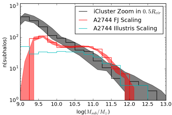
Figure 5. Comparing lensing derived SHMFs (with estimated model errors) for different assumptions relating mass to light: here we plot the SHMFs derived from the best-fit lensing model for Abell 2744 using the Faber-Jackson and Kormendy luminosity scaling laws (FJ scaling), with that derived for the best-fit lens model using the scaling laws from the full physics run of the Illustris simulations (Illustris scaling).
