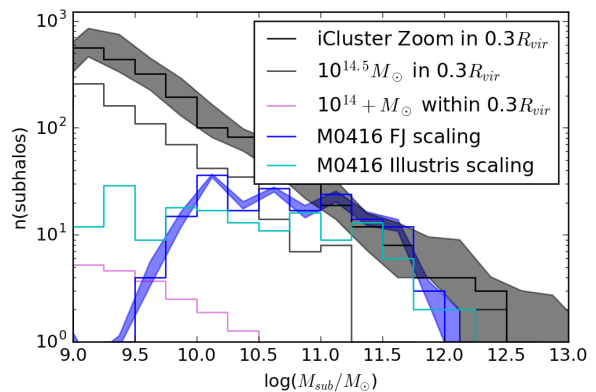
Figure 12. Comparing lensing derived SHMFs (with model errors) for different assumptions relating mass to light: here we plot the SHMFs derived from the best-fit lensing model for MACSJ0416 using the Faber-Jackson and Kormendy luminosity scaling laws, with that derived for the best-fit lens model using the scaling laws from the full physics run of iCluster Zoom 1 .
