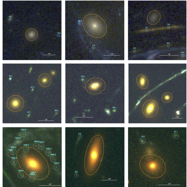
Figure 1. Low luminosity cluster member galaxies that are included in the modeling as they are required to reproduce the observed multiple image configurations. Here we show 3 panels with examples from each of the 3 clusters lenses studied here Abell 2744, MACSJ 0416 and MACSJ 1149. The deeper HSTFF data reveal fainter cluster members as well as fainter lensed sources.
