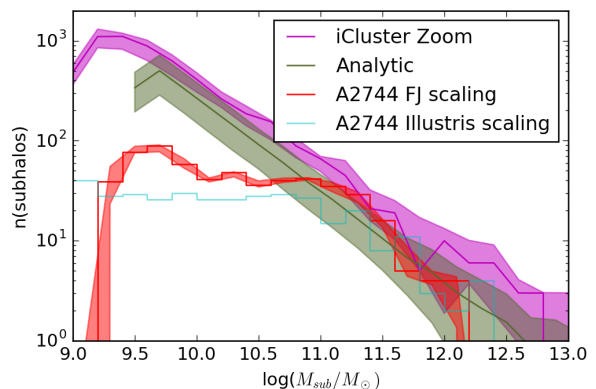
Figure 7. Comparison with the analytically predicted SHMF: the lensing derived SHMF (with model errors) for the two independent scaling laws is overplotted along with the analytically calculated SHMF for a cluster halo with mass equivalent to that of Abell 2744. This analytic estimate includes the halo-to-halo scatter that is shown in the dull green band.
