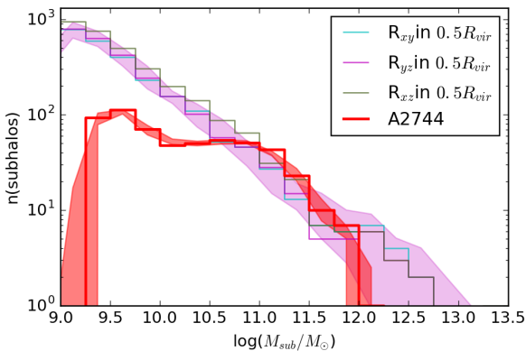
Figure 9. Projection Effects on the derived SHMF from simulations: here we plot the SHMF derived from the zoomed in Illustris cluster iCluster Zoom 1 derived by projecting along three distinct axes within 0.5 R_{\text{vir}} . Note that the dispersion arising from projection effects is negligible.
