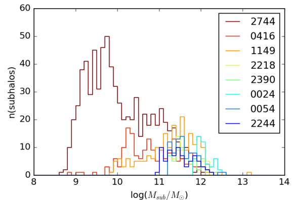
Figure 3. The comparison of the SHMF derived from our current analysis of HSTFF data for Abell 2744, MACSJ 0416 and MACSJ 1149 with prior determinations from shallower HST data for the massive lensing clusters Abell 2218, CL0024, CL0054, Abell 2390 and CL2244 that are at a similar redshift range.
