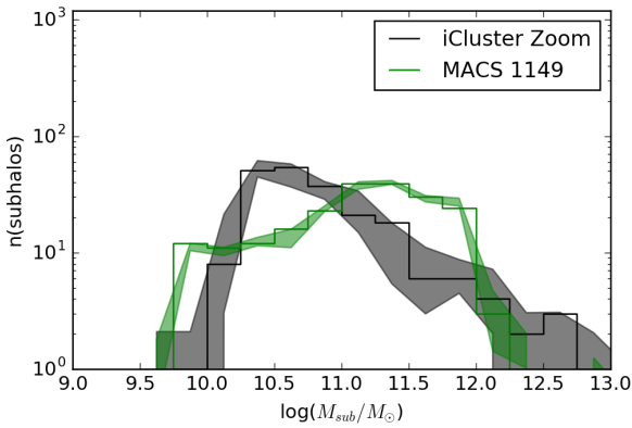
Figure 22. Comparison of the count-matched SHMF derived for MACSJ 1149 from the HST FF data (green histogram) with the iCluster Zoom 1 snapshot. Once again the iCluster Zoom 1 snapshot from the full physics run was selected, however here only the dark matter subhaloes associated with the brightest 217 cluster galaxies - number matched within 0.5R_{\text{vir}} to the HFF derived SHMF are plotted.
