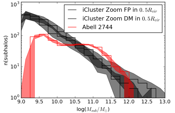
Figure 4. Comparison of the SHMF derived for Abell 2744 (with overplotted modeling errors derived from the dispersion in N-Bayesian realizations for the key fiducial parameters r_{t*} and \sigma_{0*} ) with Dark Matter only and Full Physics Illustris iCluster Zooms : The SHMF derived from the HST FF data (red histogram) for Abell 2744 is plotted along with that derived from the iCluster Zooms . The dark matter only run is plotted as a solid black histogram with the dispersion marked in the dark grey band and the full physics run (grey histogram) and corresponding dispersion shown as the light grey band. Sub haloes within 0.5 R_{vir} that corresponds to the FOV of ACS over which the lensing model has been reconstructed are extracted from iCluster Zoom 1 . The full physics run of iCluster Zoom 1 includes sub-grid models for the physical processes that are relevant to galaxy formation. From the full physics run we have selected only sub haloes that host a stellar component.
