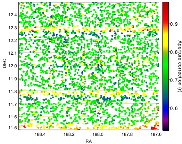
FIG. 20.— Illustration of the spatial variations of the point source aperture corrections in r , for NGVS pointing +0+0 (see Ferrarese et al. 2012 for pointing numbering). Color maps the difference between magnitudes measured in apertures of 4 and 8 pixels diameter ( 0.186''/\text{pix} ).
