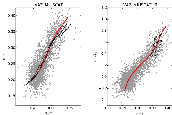
FIG. 14.— Two color-color diagrams for the Vazdekis et al. (2012) model. In the gri diagram (left panel), the symbols and lines are as in Fig. 10. In the riK diagram, the model is used with the MIUSCAT IR spectral library, for which only metallicities near solar are available. The grid nodes shown are [\text{Fe}/\text{H}] = [-0.39, 0, 0.17] .
