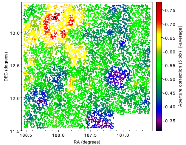
FIG. 21.— Aperture corrections for K_s point source photometry across the whole Virgo core area (thirty-four WIRCam pointings covering four MegaCam pointings).
