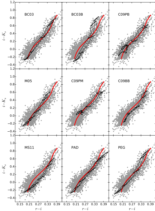
FIG. 13.— riK diagram. Symbols and lines are as in Fig. 10.
