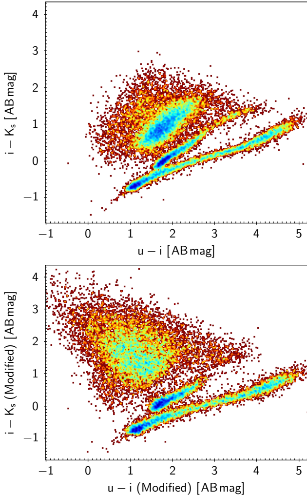
FIG. 5.— Top: the uik diagram after removing from the sample shown in Figure 4 saturated stars, large objects and sources with large errors. Bottom: the uiK diagram modified using a compactness criterion as explained in Section 3.1. The color coding in both panels maps the density of objects.
