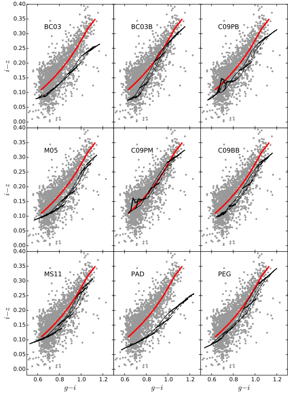
FIG. 11.— giz diagram. Symbols and lines are as in Fig. 10.
