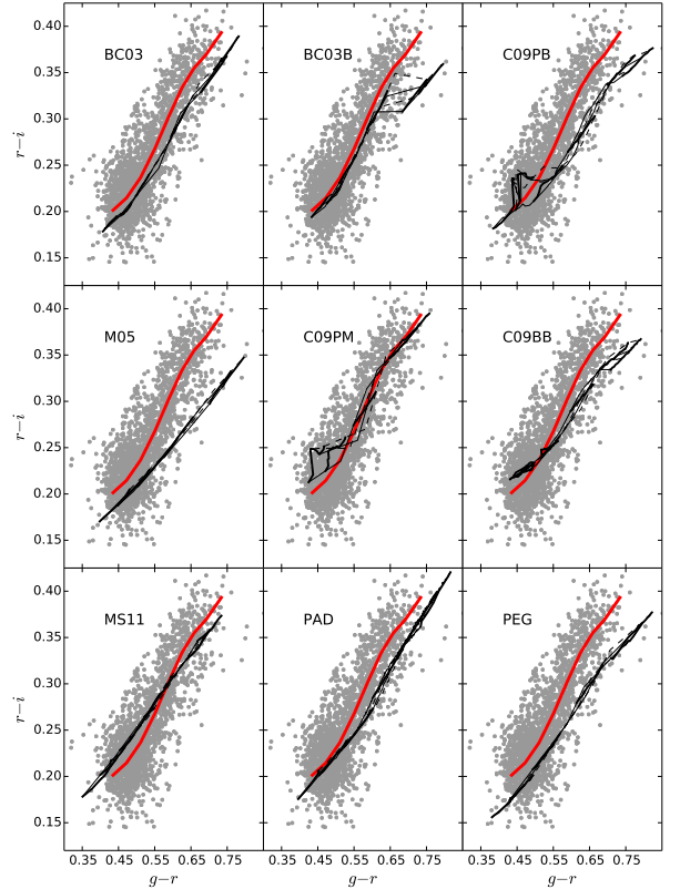
FIG. 10.— gri diagram. The gray dots are the GCs of our robust Virgo sample, after correction for foreground extinction. The calibration is that of Section 2.4 (see appendix Figure 23 for a version of these plots using the SLR calibration). For each model set, the thick solid and dashed lines represent the metallicity tracks at given ages, with metallicity increasing from the bottom left to the top right. The metallicities of the grid nodes are [\text{Fe}/\text{H}] = [-2, -1.5, -1, -0.5, 0, 0.17] (except for C09BB and C09PM, see Section 4). Alternating thin solid and dotted lines connect models of constant age, at [6, 8, 10, 13] Gyr. The red line represent the polynomial fit defined in Section 3.5. The model grids are degenerate in age and metallicity in this particular color-color diagram.
