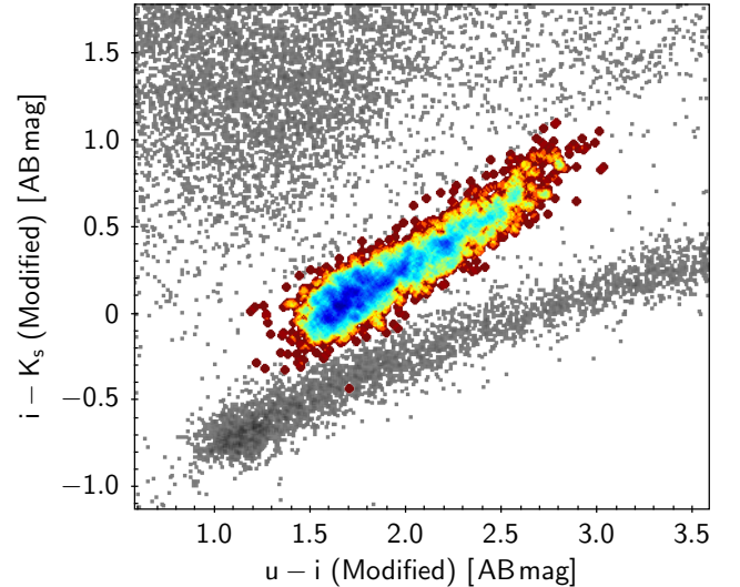
FIG. 6.— Final selection of the NGVS GCs in the modified uiK diagram. The color coding for the GC maps the density of objects.
