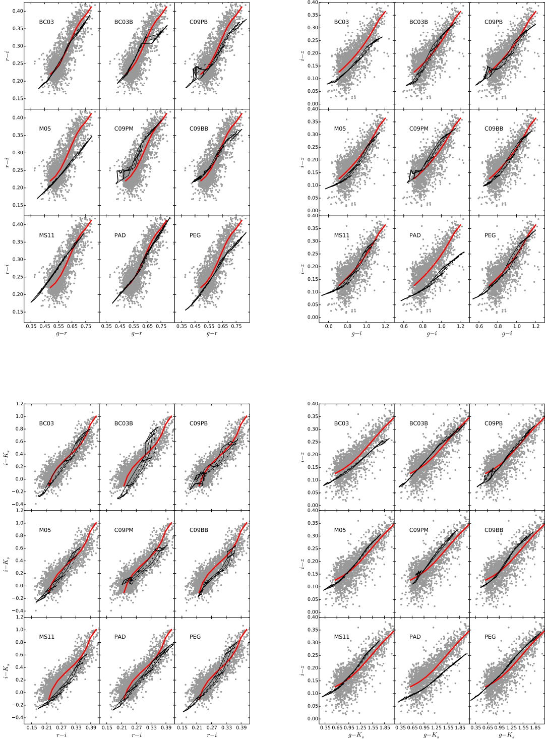
FIG. 23.— Virgo core GC color-color diagrams with SLR-based photometry. The symbols and lines are as in Fig. 10.
