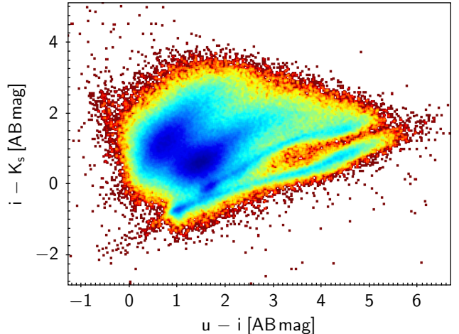
FIG. 4.— NGVS pilot-field detections in the uiK diagram. The colors shown are from measurements in 8 pixel diameter apertures ( 1.48'' ) to which point source aperture corrections are applied (i.e. they are representative only of central colors for extended sources). Most sources are background galaxies. The foreground stars are mainly along the bottom sequence, and the globular clusters are located just above it and below the two large regions of galaxies. At the red end of the GC sequence ( u - i > 3 ), redshifted passively evolving galaxies are found. The color coding maps the density of objects.
