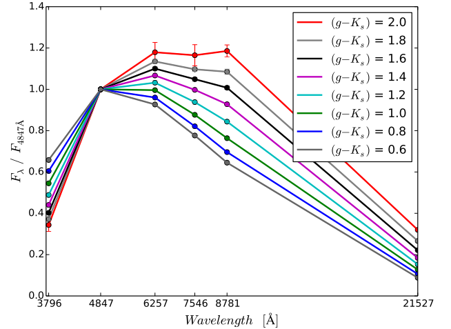
FIG. 9.— Fiducial SEDs for the NGVS globular cluster sample described in Section 3. The corresponding values of (g - K_s) [AB] are indicated. They are representative of the range of GC metallicities. These SEDs are available in Tab. 4.
