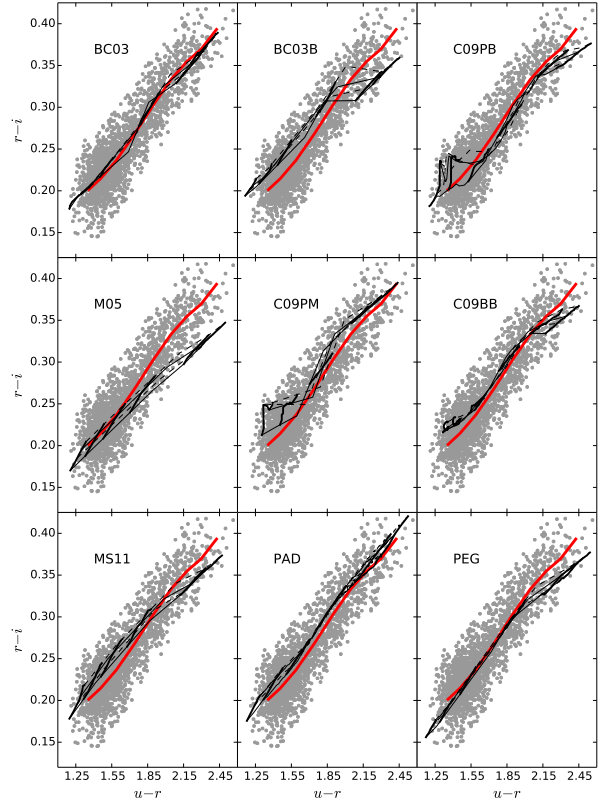
FIG. 15.— uri diagram. Symbols and lines are as in Fig. 10.
