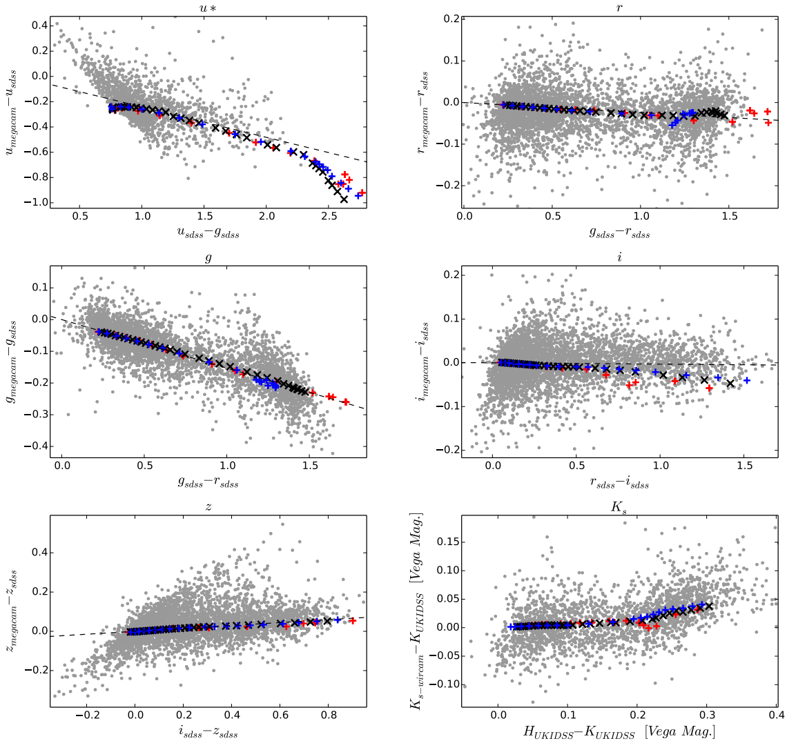
FIG. 1.— Transformation between photometric systems. Star in common between NGVS and SDSS, or NGVS and UKIDSS (for K_s ) are shown as grey dots. For NGVS and UKIDSS, aperture corrected magnitudes are used; for SDSS, psf magnitudes are adopted. The NGVS magnitudes are the final values obtained as described in Section 2.4. In each panel, a different subset of stars is plotted, restricted so the SDSS or UKIDSS magnitudes used in the panel have errors as follows: \sigma(u^*) < 0.20 , \sigma(g) < 0.10 , \sigma(r) < 0.10 , \sigma(i) < 0.10 , \sigma(z) < 0.15 , \sigma(H_{UKIDSS} - K_{UKIDSS}) < 0.04 mag. Synthetic photometry based on model dwarf stars is shown with crosses, based on energy distributions from MARCS models (blue), PHOENIX models (black) and the BaSeL library (red). Along these sequences, stellar parameters are taken from the Besançon model of the Milky Way. The dashed lines in the five first panels follow the equations quoted in Ferrarese et al. (2012).
