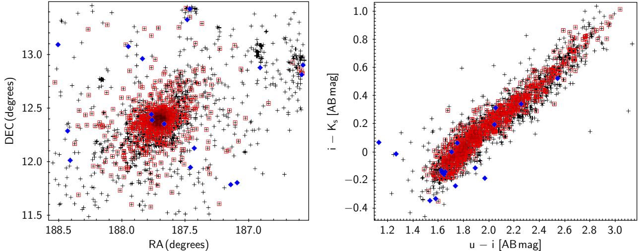
FIG. 7.— Left: Selected NGVS GC candidates from our modified uiK diagram (black), spectroscopically confirmed GCs based on matching to literature data (red), and the false positive matches (blue). Right: the NGVS GC candidates in the uiK diagram (black), spectroscopically confirmed GCs matched to the literature (red), and the false positive matches (blue).
