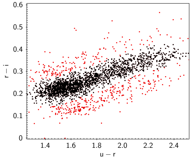
FIG. 8.— The r band issues caused by different seeing in the 0-0 tile plotted in the uri diagram. The 2 external and mistaken branches are highlighted in red.
