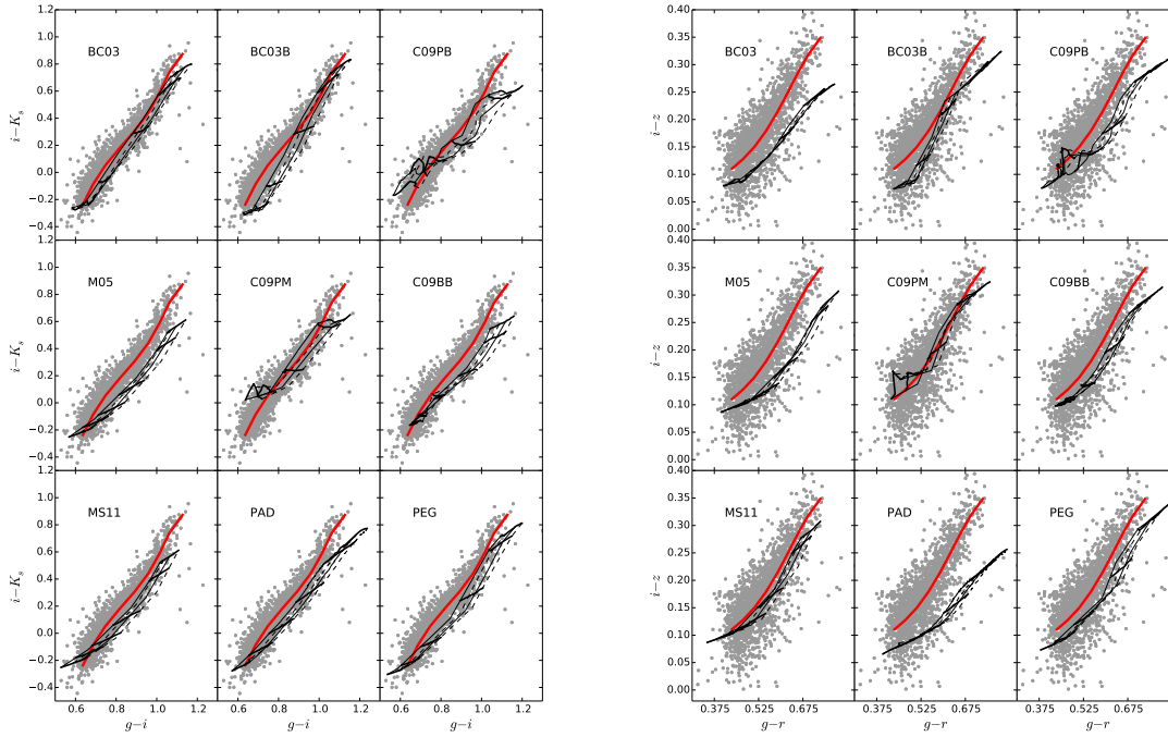
FIG. 24.— The giK and griz diagrams of Virgo core GCs, with NGVS photometry calibrated against external catalogs. The symbols and lines are as in Fig. 10.
