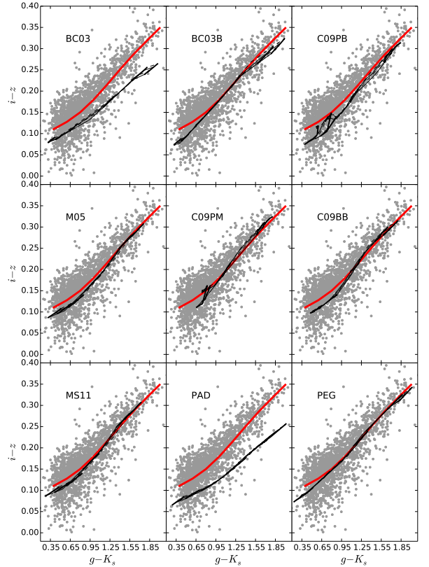
FIG. 12.— gKiz diagram. Symbols and lines are as in Fig. 10.
