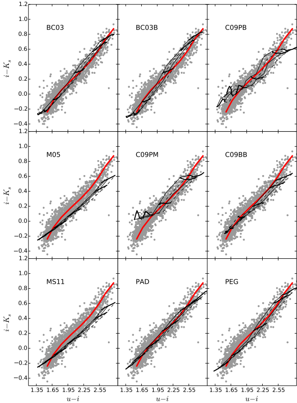
FIG. 16.— uiK diagram. Symbols and lines are as in Fig. 10.
