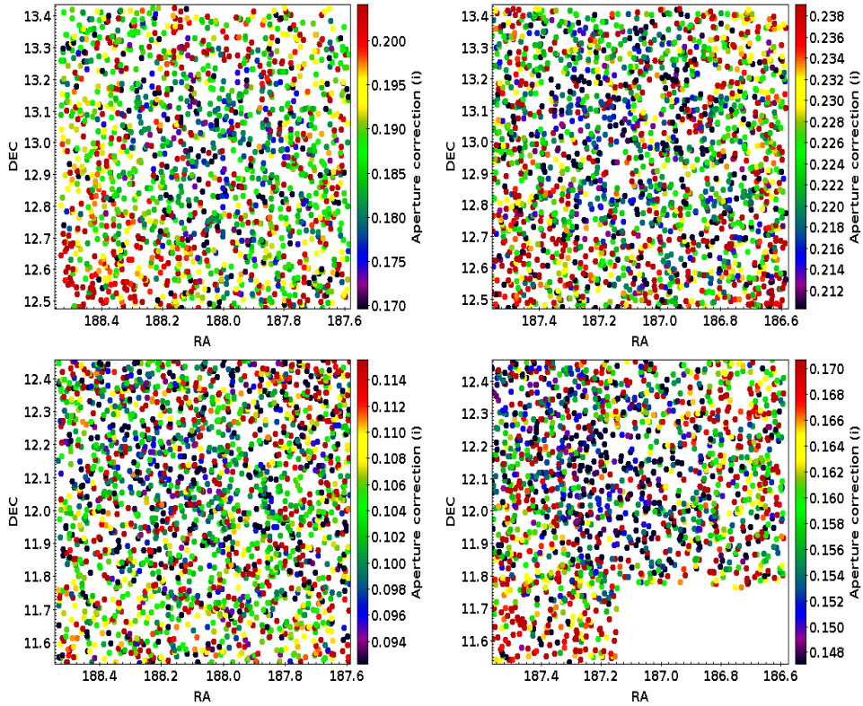
FIG. 19.— Illustration of the spatial variations of the point source aperture corrections in i within individual pointings. From left to right, then top to bottom, the fields correspond to NGVS MegaCam pointings +0+1, -1+1, +0+0, and -1+0 (Ferrarese et al. 2012).
