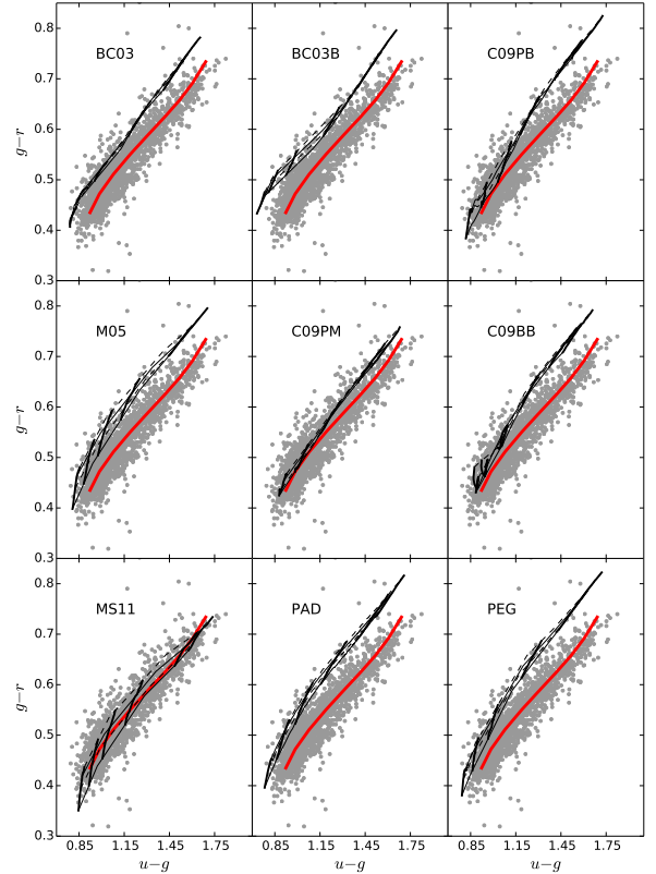
FIG. 17.— ugr diagram. Symbols and lines are as in Fig. 10.
