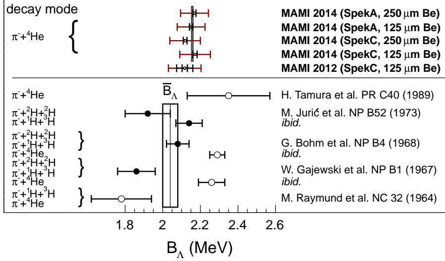
Figure 4: \Lambda binding energies of {}^4_{\Lambda}\text{H} from decay-pion measurements [3, 16–19]. The binding energy value from Ref. [16] was calculated from the observed momentum. Errors on the emulsion data are statistical only. The mean value as compiled by Ref. [3] excludes data from the two-body decay mode and is represented by the error band. The uncertainties on the MAMI value are statistical (inner) and total (outer), where the total error is the sum of the statistical one and the systematic one in quadrature. The MAMI 2012 data set has an additional error (middle) of \sim 30 keV due to the instability of the magnetic field.
