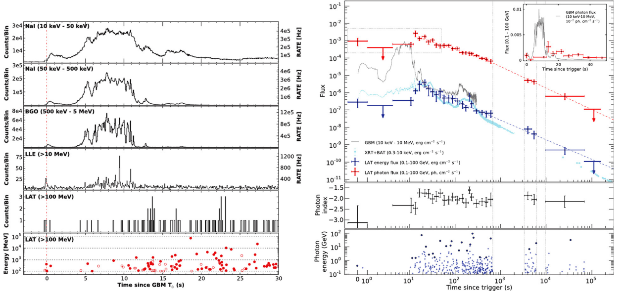
Fig. 5. Left: GRB 130427A light curves as measured by the Fermi/GBM and the Fermi/LAT [31] (see caption of Fig. 3, left). Right: GRB 130427A energy flux light curves (in \text{erg cm}^{-2} \text{s}^{-1} = 10^{-3} \text{ W m}^{-2} ) as measured by Fermi (GBM and LAT instruments) and Swift (BAT and XRT instruments) [31]. The second panel shows the spectral index \alpha_{\text{EX}} of the high-energy power law, and the last panel displays the energies of the individual photons which are well reconstructed by the LAT above 100 MeV.
