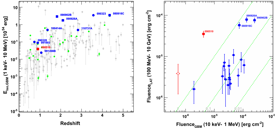
Fig. 6. Left: Isotropic equivalent energy E_{\text{iso}} (in \text{erg} = 10^{-7} \text{ J} ) in the source frame energy range [E'_1, E'_2] = [1 \text{ keV}, 10 \text{ MeV}] as a function of the redshift for all the GRBs with measured distance in the first Fermi/LAT catalog [26], compared to the GRBs in the Swift/BAT [33] (in gray) and Fermi/GBM [19] (in green) catalogs. Right: Fluence (in \text{erg cm}^{-2} = 10^{-3} \text{ J m}^{-2} ) as measured by the Fermi/GBM (10 keV–1 MeV) vs. that measured by the Fermi/LAT (> 100 MeV) during their respective T_{90} 's (Fig. 7, right) for all GRBs in the first Fermi/LAT catalog [26]. In both panels, long GRBs are displayed in blue, and short GRBs in red.
