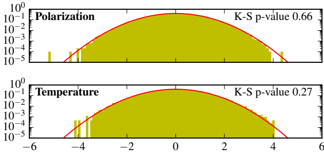
Fig. 2. Histogram of the whitened unbiased map \mathbf{V}\text{diag}(\sqrt{\hat{\epsilon}})\mathbf{V}^T\hat{\delta} , where \hat{\delta} is estimated starting from a time-domain white noise simulation (see Sect. 5.5 for the details).
