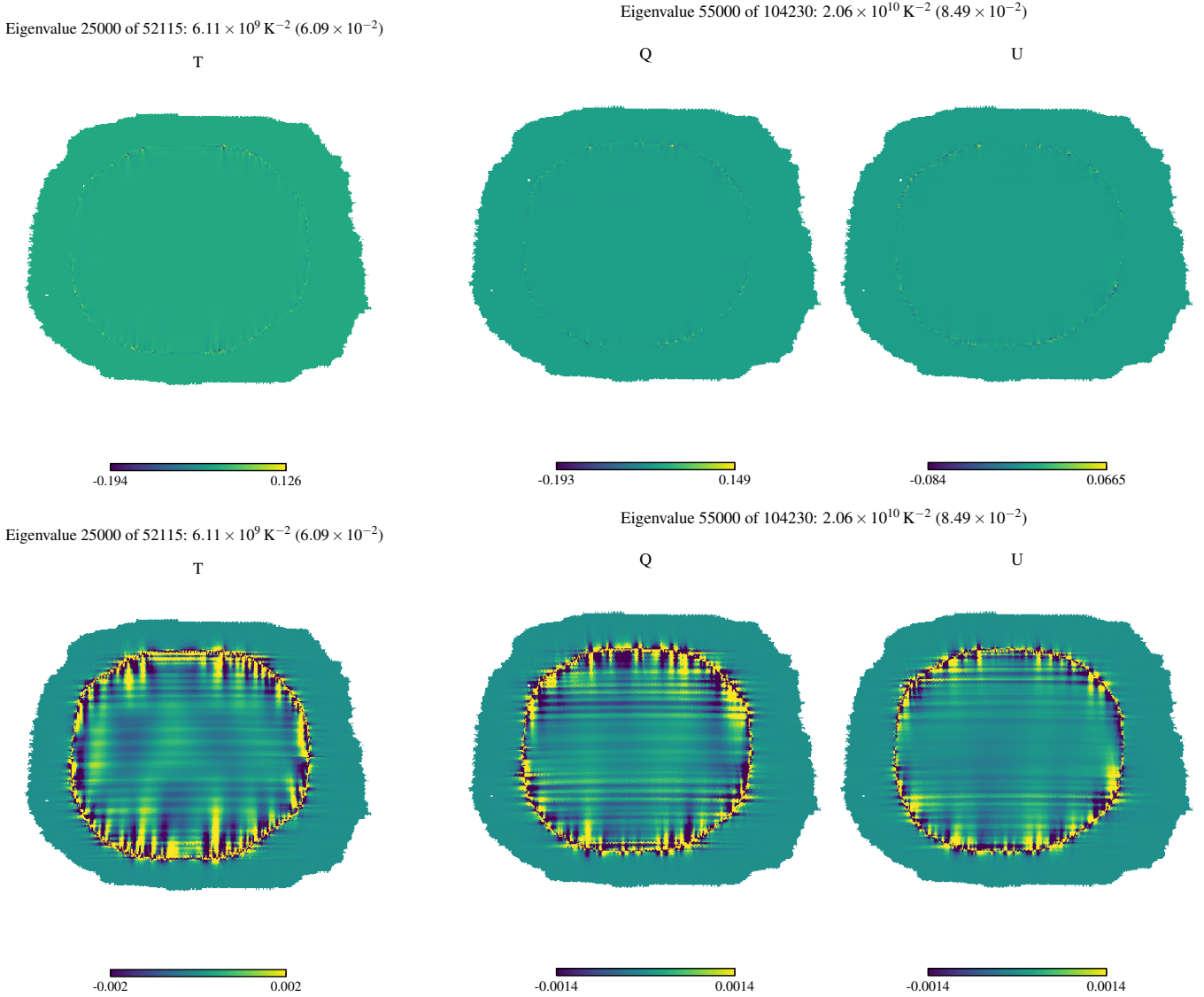
Fig. 11. Examples of pixel-like modes (the parenthesis in the title reports the corresponding eigenvalue divided by the largest eigenvalue). These modes involve mainly a “ring” composed of a very limited number of pixels (see the first row ). In the second row , the same eigenvectors are displayed with a color scale squeezed by roughly two orders of magnitude, emphasizing structures inside and outside of the ring. Outside of the ring the structures quickly fade away. Also moving inwards the structures decrease their amplitude. However, compared to the outward structure, their typical length is much larger and, most important, they do not completely disappear: they have a relevant amplitude in the whole inner region. We emphasize that the “horizontal” structures represent the correlations induced by the ground template filtering.
