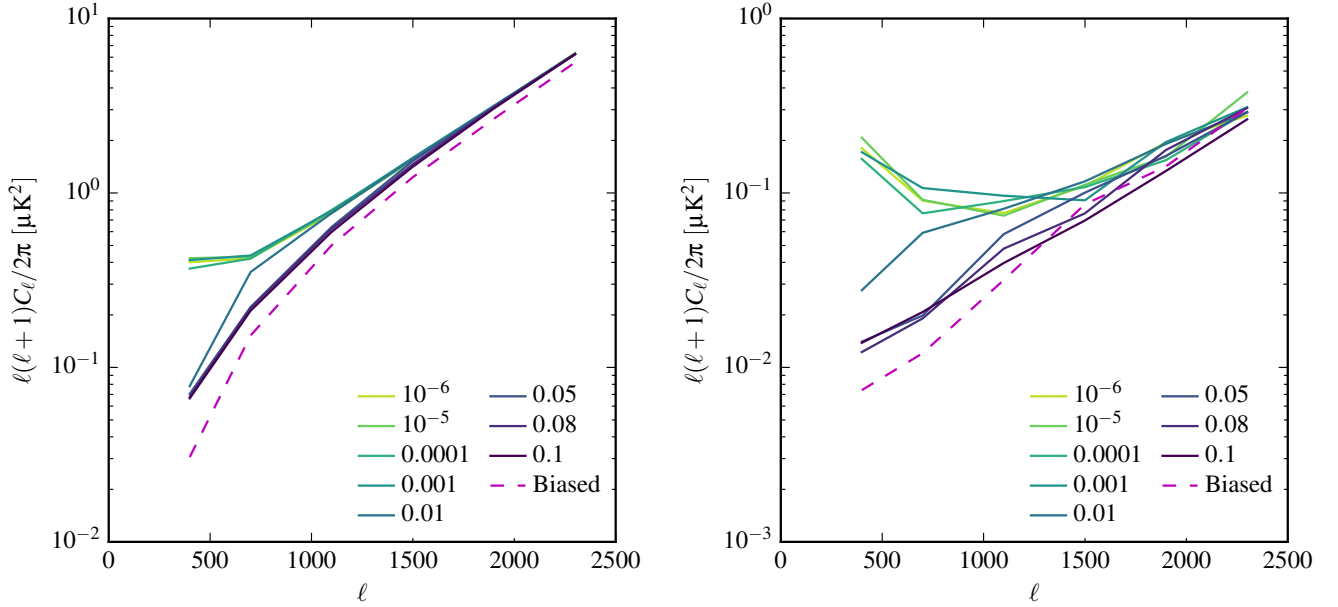
Fig. 12. Mean ( left ) and standard deviation ( right ) of the B -mode power spectra (as computed by X^2\text{PURE} ) of 100 noise only simulations for different input maps. “Biased” refers to the biased map estimator defined in Eq. (25). The other lines refer to different maps derived from the unbiased map estimator Eq. (22). The value in the legend is the \alpha parameter that quantifies the amount of map domain filtering applied to the unbiased map. Higher values of \alpha correspond to more aggressive filtering, see Sect. 6.3.1 for more details.
