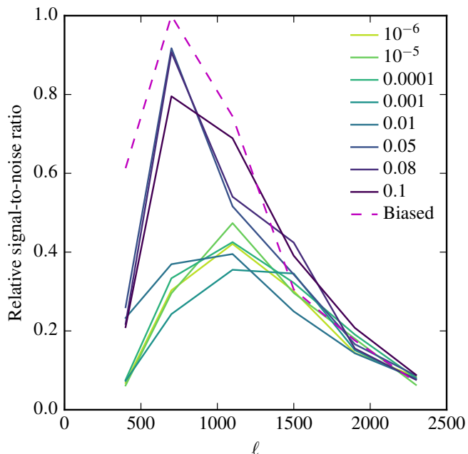
Fig. 15. Ratio between the signal and the total uncertainty for B -mode power spectra derived with the different power spectrum estimation choices. The results are quoted relative to the highest ratio obtained from the unbiased map is apparent and related to the strong correlated noise modes present in the map. The loss can be mostly recovered with help of a progressively more aggressive removal of the noisiest modes as expressed by the increasing value of parameter \alpha as defined in the text and given in the legend.
