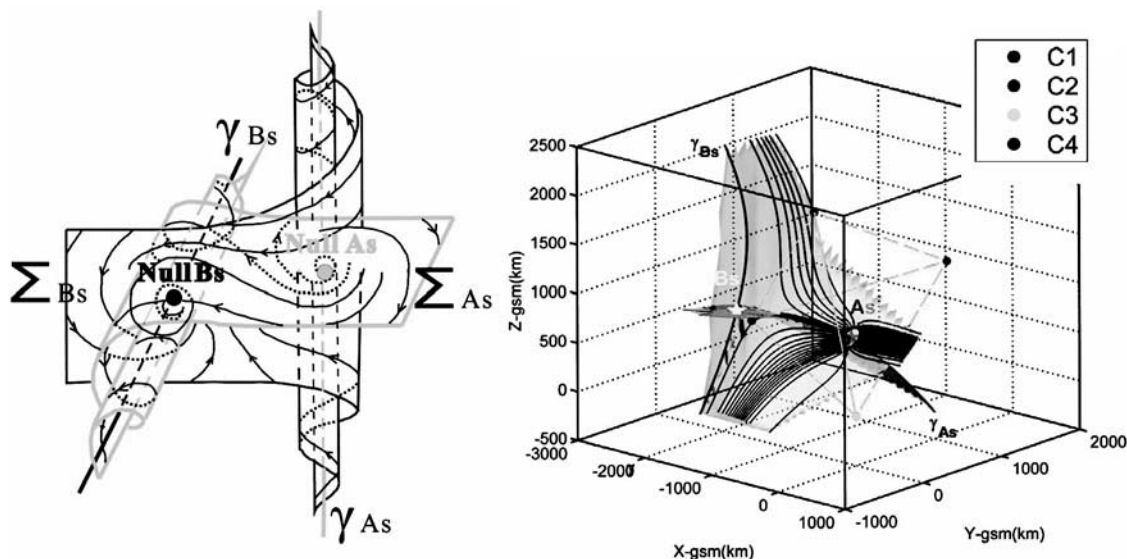
Figure 2. Three-dimensional reconnection structures. The left part is the structure of the spiral null pair of negative spiral null point A_s and positive spiral null point B_s . The fan surface of the spiral null A_s wraps the spine of the spiral null B_s whereas the fan surface of B_s wraps the spine of A_s . The right part is the structure of the magnetic field lines near the null A_s and null B_s at the time of 09:48:05 UT obtained by the fitting method. There are spiral structures near null A_s and null B_s . Near the null B_s , the spine \gamma_{B_s} of null B_s approaches the magnetic field lines in the fan surface \Sigma_{A_s} of null A_s , and near the null A_s , the \gamma_{A_s} approaches the magnetic field lines in the fan surface \Sigma_{B_s} . The angles between the spines and fans are 2.4^\circ and 1.3^\circ , respectively.
