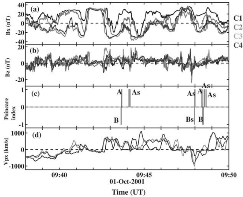
Figure 1. Cluster measurements and calculated Poincaré index during the interval of 09:38–09:50 UT on 1 October 2001. From top to bottom: Components of the magnetic field (FGM) (a) Bx and (b) Bz, (c) the Poincaré index, and (d) X component of the proton bulk velocity (CIS) versus time in the GSM coordinate system.
