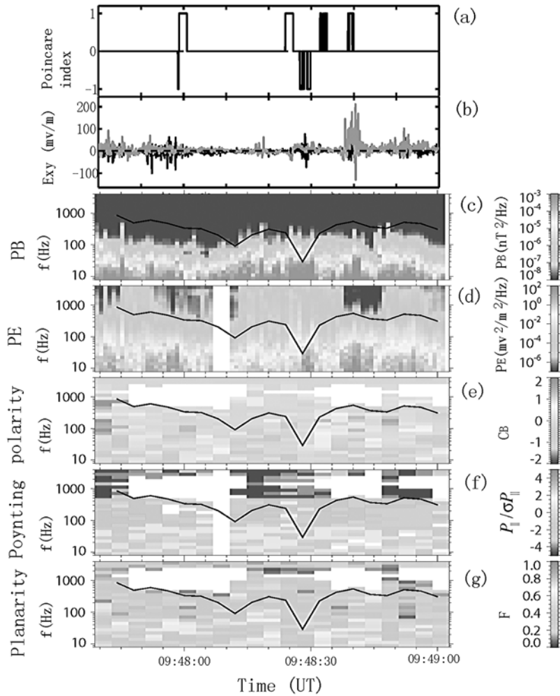
Figure 4. Wave characteristics observed by C2 during the period of 09:47:40–09:49:00 UT on 1 October 2001. From top to bottom are (a) the Poincaré index, (b) the X and Y components of electric fields, (c, d) power-spectral densities of magnetic and electric fields, and (e) the indicator of the sense of polarization. For the left circularly polarized field, the ellipticity is -1 , a value of +1 corresponds to the right circular polarization. A linearly polarized field has a zero ellipticity. (f) Normalized component of the Poynting vector parallel to the ambient magnetic field, and (g) the planarity of the magnetic field polarization. Solid lines on the dynamic spectra show the electron cyclotron frequency.
