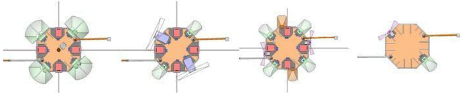
Fig. 6 Accommodation and fields of view of the scientific payload on the electron (left), ion (two middle), and fluid-scale (right) spacecraft [1]. Table 1 identifies the instruments and bay locations, which are lettered in Fig. 5
