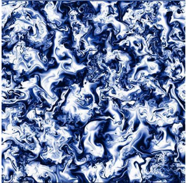
Fig. 3 A computer simulation of 2D electron MHD turbulence, showing how plasma currents are spatially localised into thin sheets and whorls. Many-point measurements, such as those from Cross-Scale, are required to measure such structures in 3D in space plasmas over a range of scales not accessible in simulations [after 4]
