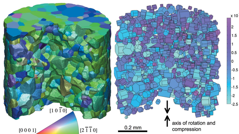
Figure 12 Grain shapes, orientations and elastic strain measured simultaneously in a single DCT scan of a pure Ti specimen. The sample exhibits a strong texture and is loaded in compression. The three-dimensional grain map is coloured according to the orientations in the inverse pole figure (left). The same grain locations, orientations and sizes are represented by hexagonal unit cells and colour coded according to the normal strain along the rotation axis and loading direction (right). A quarter of the grains were rendered invisible for better visualization of the internal grain boundaries.
