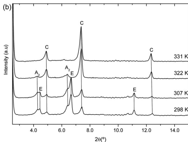
Fig. 4 (a) DSC analysis at 2 K min -1 and (b) powder X ray diffraction patterns at increasing temperatures of a mixture of E, A 2 and C forms in a sample of C 16 H 31 O 2 H. The inset in part (a) shows the first order solid solid transitions from each individual form to the C form during the first heating process (solid line). Solid solid transformations are not observed during the second heating process (dotted line).
