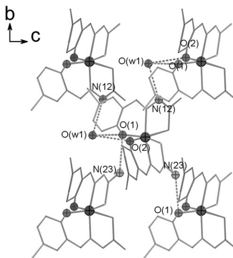
Fig. 5 Strongest intermolecular contacts between complexes at 373 K.
