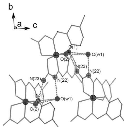
Fig. 6 Strongest intermolecular contacts between complexes at 150 K.
