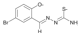
Chart 1 \text{5BrThsa}^{2-} ligand.
