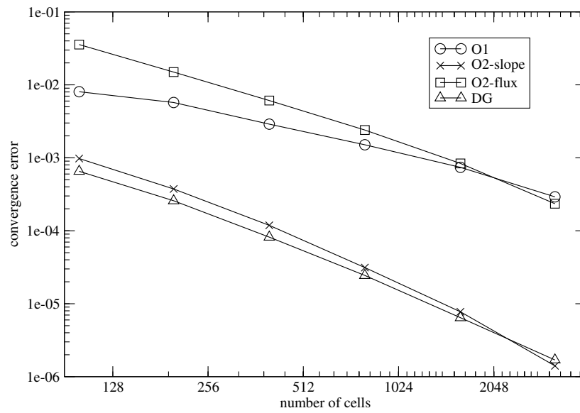
Figure 7: 1D Couette flow: convergence rates of the discontinuous Galerkin and finite volume schemes with uniform meshes, for the heat flux.
