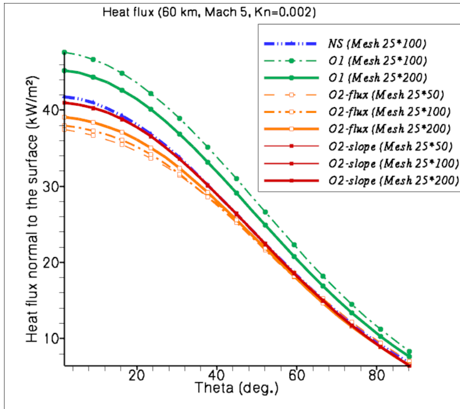
Figure 5: 2D supersonic flow: comparison of the heat flux between BGK solved with finite volume schemes (O1, O2-flux, O2-slope) for different meshes, and Navier-Stokes (NS)
