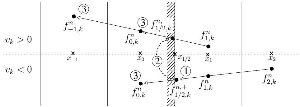
Figure 1: Finite volume scheme: definition of the ghost cell values f_{0,k}^n and f_{-1,k}^n by using linear extrapolations and the boundary condition.
