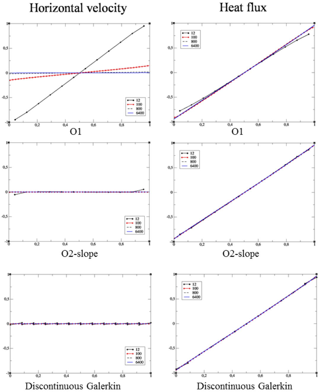
Figure 5: 1D Couette flow: results obtained with the discontinuous Galerkin scheme and first and second order finite volume schemes for the horizontal velocity and the heat flux, with 12 to 6400 grid points.
