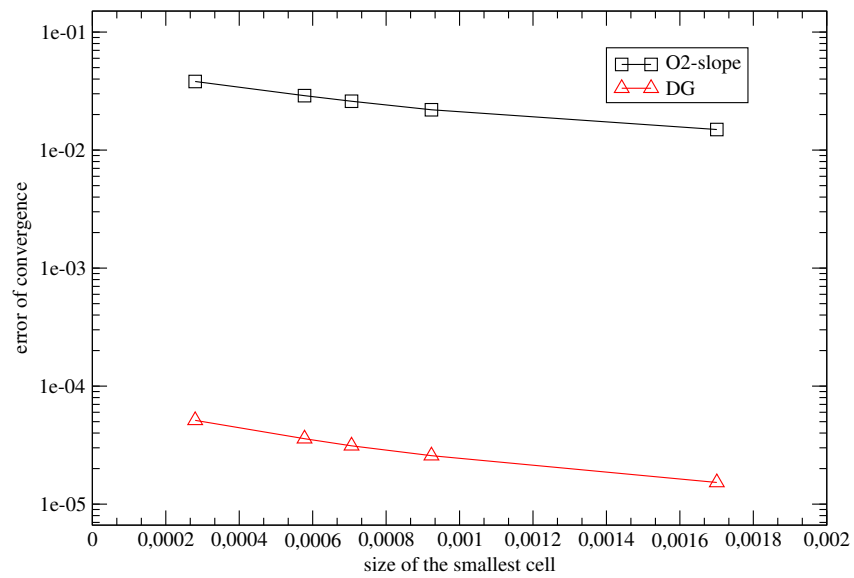
Figure 7: 1D Couette flow: convergence rate of the discontinuous Galerkin and finite volume schemes for refined meshes (heat flux at the wall)
