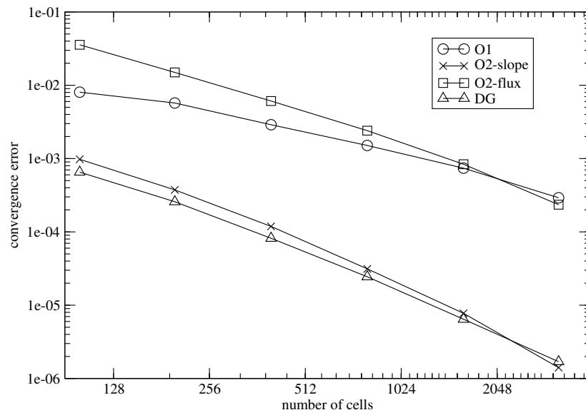
Figure 6: 1D Couette flow: convergence rates of the discontinuous Galerkin and finite volume schemes with uniform meshes, for the heat flux
