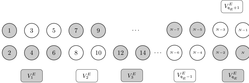
Figure 3: Elements of \mathcal{V}^E , case n = 3 , r_E = 0 .
