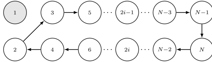
(b) Round-robin permutation.
