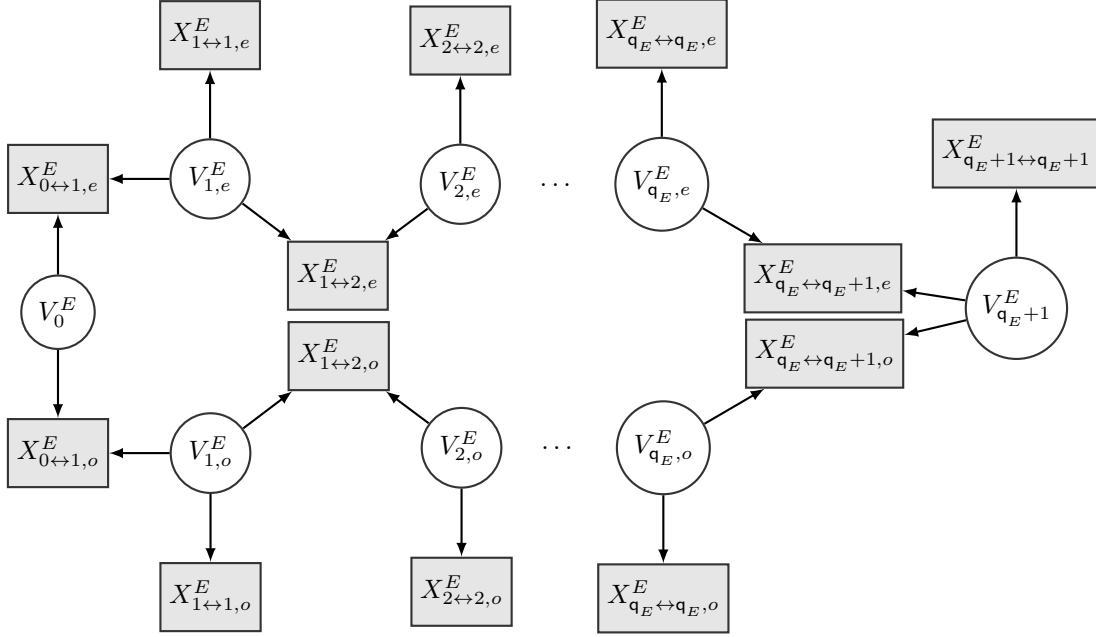
Figure 5: Graphical model of the round-robin algorithm.
