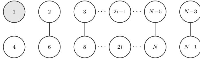
(c) Round-robin pairing, step 2.
