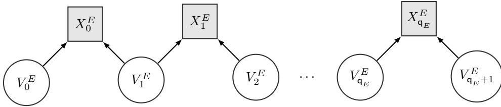
Figure 2: Graphical model of paired comparisons contests.
