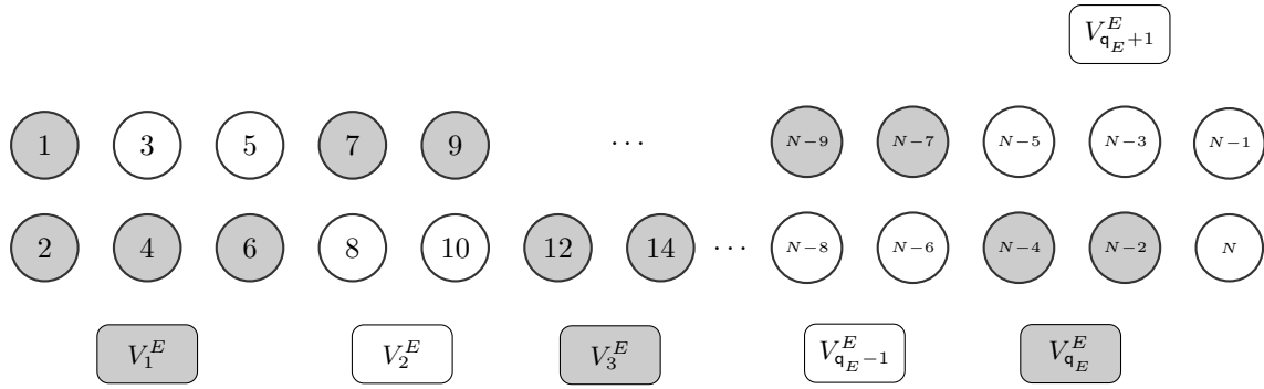
Figure 4: Elements of \mathcal{V}^E , case n = 3 , r_E = 1 .
