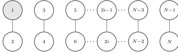
(a) Round-robin pairing, step 1.
