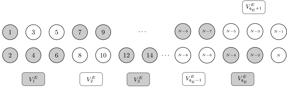
Figure 4: Elements of \mathcal{V}^E , case n = 3 , r_E = 1 .
