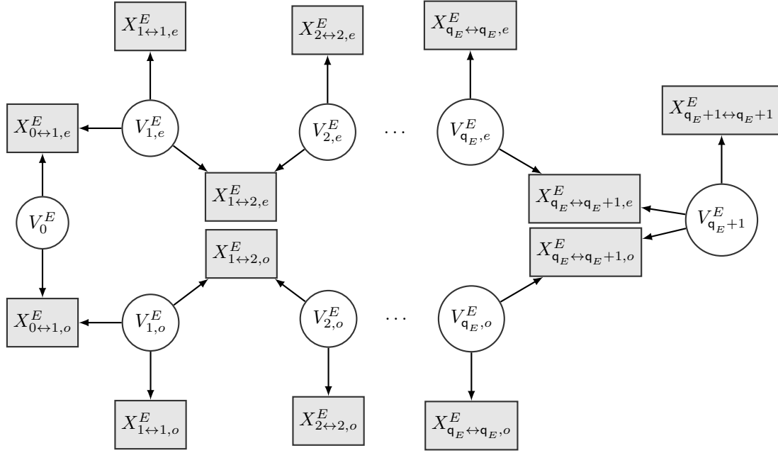
Figure 5: Graphical model of the round-robin algorithm.
