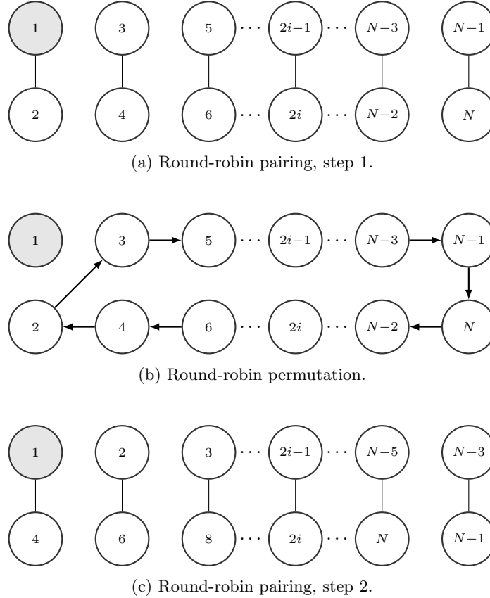
Figure 1: Round-robin algorithm.
