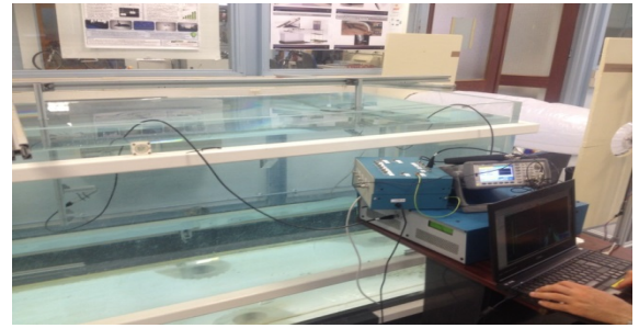
Fig. 3. Experimental facility.
