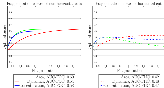
Fig. 4. Fragmentation curves of non-horizontal and horizontal cuts of the concatenation of area and dynamics based watershed hierarchies. The 10 th highest levels of area were concatenated to the lower level sets of the dynamics based hierarchy.
