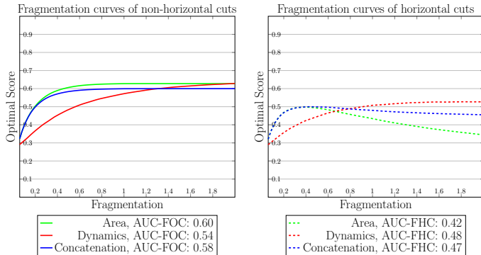
Fig. 4. Fragmentation curves of non-horizontal and horizontal cuts of the concatenation of area and dynamics based watershed hierarchies. The 10 th highest levels of area were concatenated to the lower level sets of the dynamics based hierarchy.
