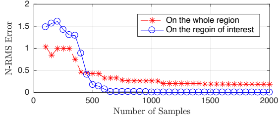
Fig. 6: The N-RMS error of the estimation of the nonlinear model of [\mathbf{J}_g(\mathbf{x})]_{1,1} with respect to the number of samples over 1) a M \times M square (the dashed line) and 2) the region of interest in which the samples exist (the solid line)
