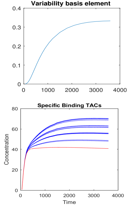
Fig. 4. Top: variability basis element \mathbf{v}_1 identified by PCA. Bottom: generated SBE TACs (blue) and the nominal SBE signature (red).
