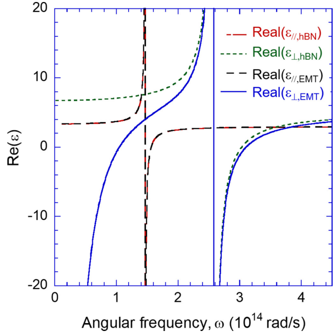
FIG. 6. Dielectric functions of hBN and the effective dielectric functions of the multilayer structure based on Eq. (12). The parameters are h = 50 nm and \mu = 0.3 eV.
