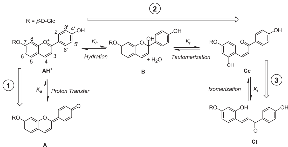
Scheme 1. Multistate of the 7- \beta -D-glucopyranosyloxy-4'-hydroxyflavylium ion. Sequence of reactions after a direct pH jump (observed in anthocyanins and other flavylium-based multistates exhibiting a high cis-trans isomerization barrier). Three kinetic steps can be differentiated: 1- Proton transfer which occurs in the \mu s time scale; 2- rate limiting hydration (seconds-minutes time scale) followed by fast and therefore kinetically silent tautomerization and 3- slow isomerization in the hours time scale.
