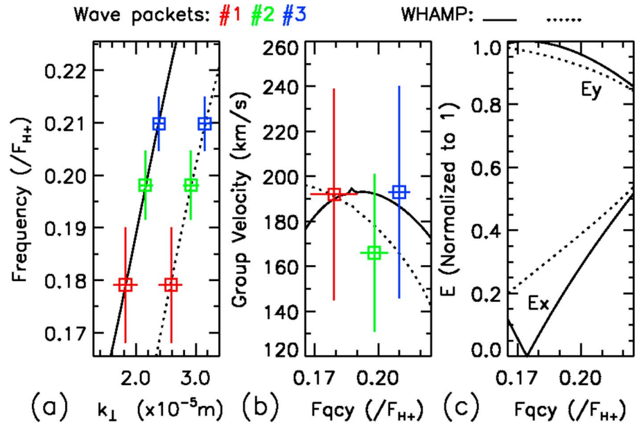
Figure 4. Comparison of observations (colored squares and lines) to numerical computation results for two different plasma compositions: (n_{H^+}; n_{He^+}; n_{O^+})_1 = (460; 70; 70) \text{ cm}^{-3} (plain black lines) and (n_{H^+}; n_{He^+}; n_{O^+})_2 = (1140; 110; 50) \text{ cm}^{-3} (dotted black lines). Frequency versus k_{\perp} , group velocity versus frequency, and perpendicular electric field components versus frequency.
