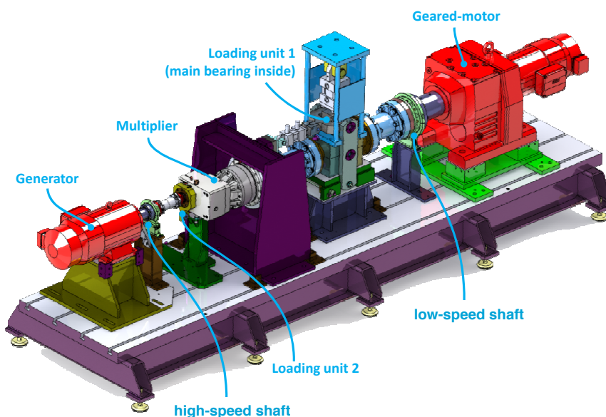
Figure 7: Structure of the test bench used for bearing faults monitoring [17].
