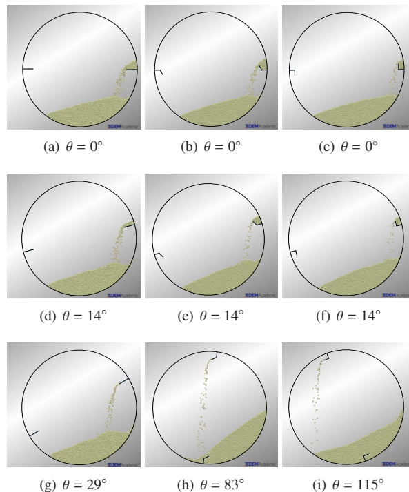
Figure 5. Snapshots of the granular behaviour in the rotating drum for three shapes of the flight
