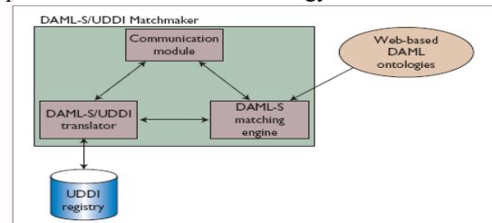
Fig. 5. DAML/S/UDDI matchmaker
