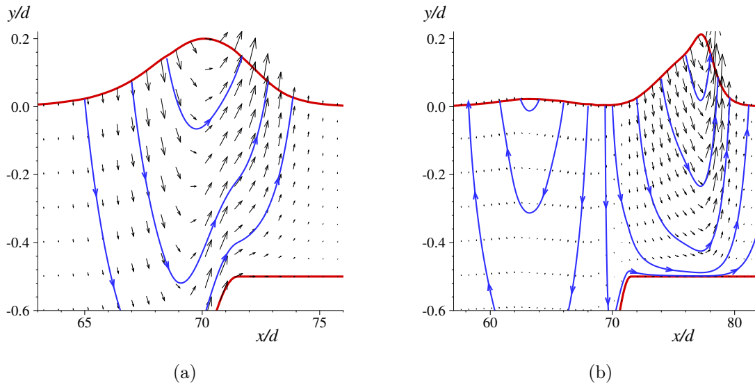
Figure 11. Reconstructed velocity field in the fluid during the solitary wave interaction process with an underwater step: (a) t = 2.0 s, (b) t = 3.0 s. Solid blue lines show a few streamlines. Numerical parameters are provided in Table 2.
