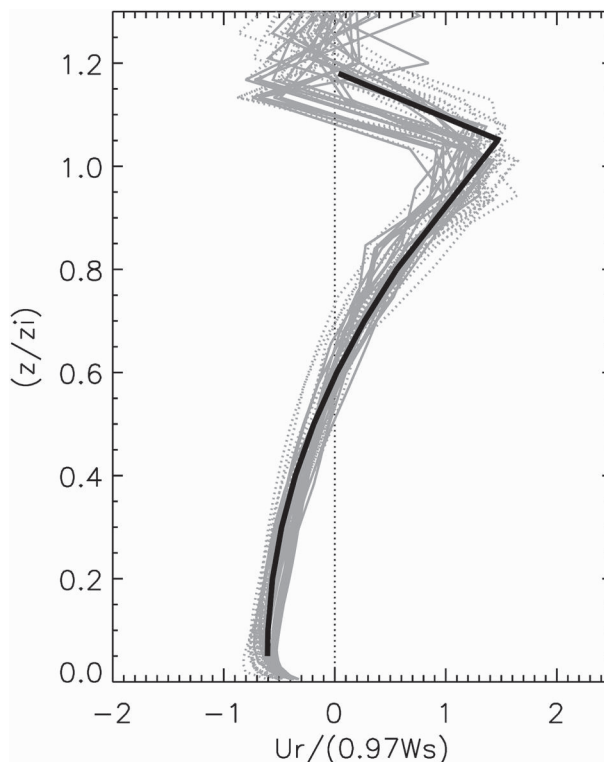
FIG. 8. Normalized profiles of radial velocity U_r . The continuous gray lines correspond to the simulation for D = 10 km, the dotted gray lines correspond to the simulation for D = 20 km, and the black lines represent the best least squares polynomial fit.
