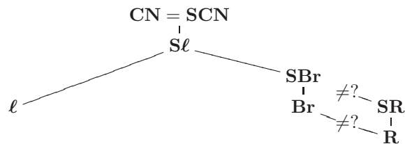
FIGURE 1.1. Classes of completely normal spectral spaces
