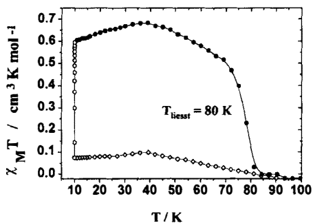
Figure 6. \chi_{\text{M}}T versus T plots for \text{Fe}(\text{PM-BiA})_2(\text{NCS})_2 in phase I; ( \diamond \diamond \diamond ) without irradiation, ( \circ \circ \circ ) under irradiation at 10 K and ( \bullet \bullet \bullet ) under irradiation.
