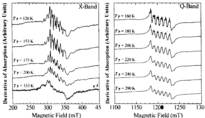
Figure 4. X- and Q-bands EPR spectra of the intentionally doped Fe_{0.99}Mn_{0.01}(PM-BiA)_2(NCS)_2 .
