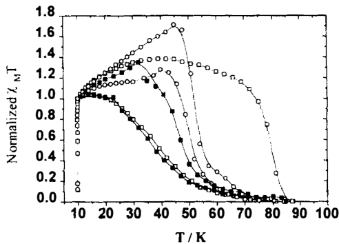
Figure 7. Magnetic properties recorded under light irradiation for (□ □ □) in phase I, (○ ○ ○) in phase II and (■ ■ ■) for \text{Fe}_{0.216}\text{Mn}_{0.784}(\text{PM-BiA})_2(\text{NCS})_2 .
