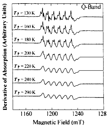
Figure 3. Q-band EPR spectra of the naturally doped Fe(PM-BiA)_2(NCS)_2 in phase II in the warming ( T \uparrow ) mode.
