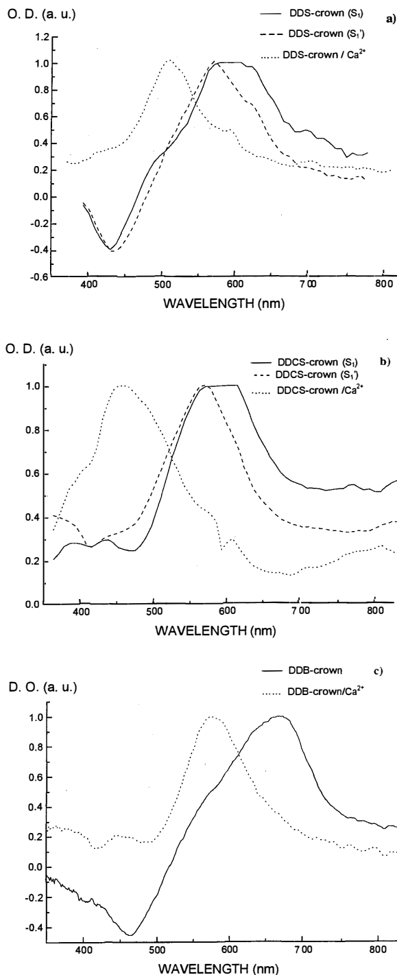
Figure 4. – Transient absorption spectra of the three probes in acetonitrile. Without \text{Ca}^{2+} : full line (first excited state S_1 ), dashed line (second intermediate state S'_1 ). With \text{Ca}^{2+} : dotted line. (a) DDS-crown, (b) DDCS-crown and (c) DDB-crown.
