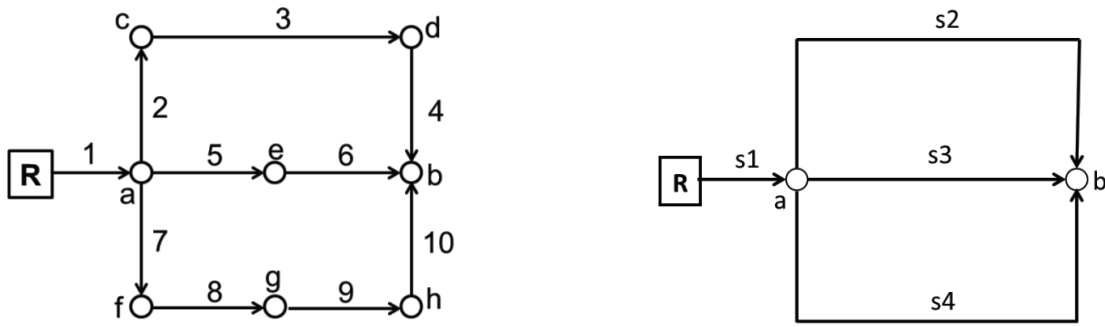
Fig. 1. (a) example system; (b) and its topological minor (supernodes and superlinks).
