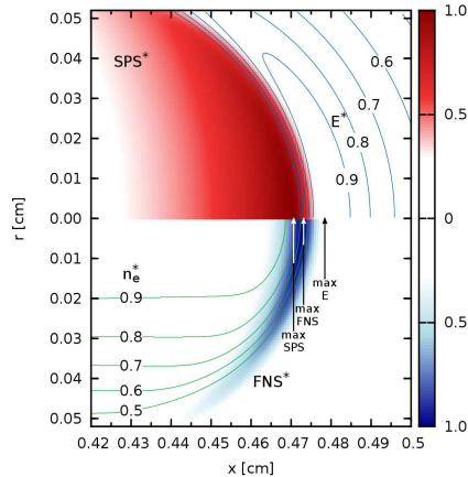
Figure 6: Detailed view on the positive streamer head structure obtained from 2D axisymmetric simulation. In upper part, electric field isolines and emission profile of SPS (red) are shown. In the part below, electron density isolines and emission profile of FNS (blue) are presented. The star-signs denote a normalised value. Note, that while the results of measurements on the streamer discharge are typically represented in the time scale of measured temporal development, i.e. from left to the right as in Fig. 2 or in [16,29,36,38], the results of numerical modelling are presented in opposite direction [15,17], which is also the case further in this article.
