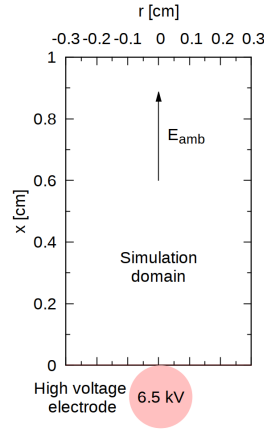
Figure 4: Simulation domain: High voltage electrode is a conducting sphere of radius 0.1 \text{ cm} and voltage 6.5 \text{ kV} . Homogeneous ambient electric field E_{amb} of 12 \text{ kVcm}^{-1} is established by remote planar electrodes.
