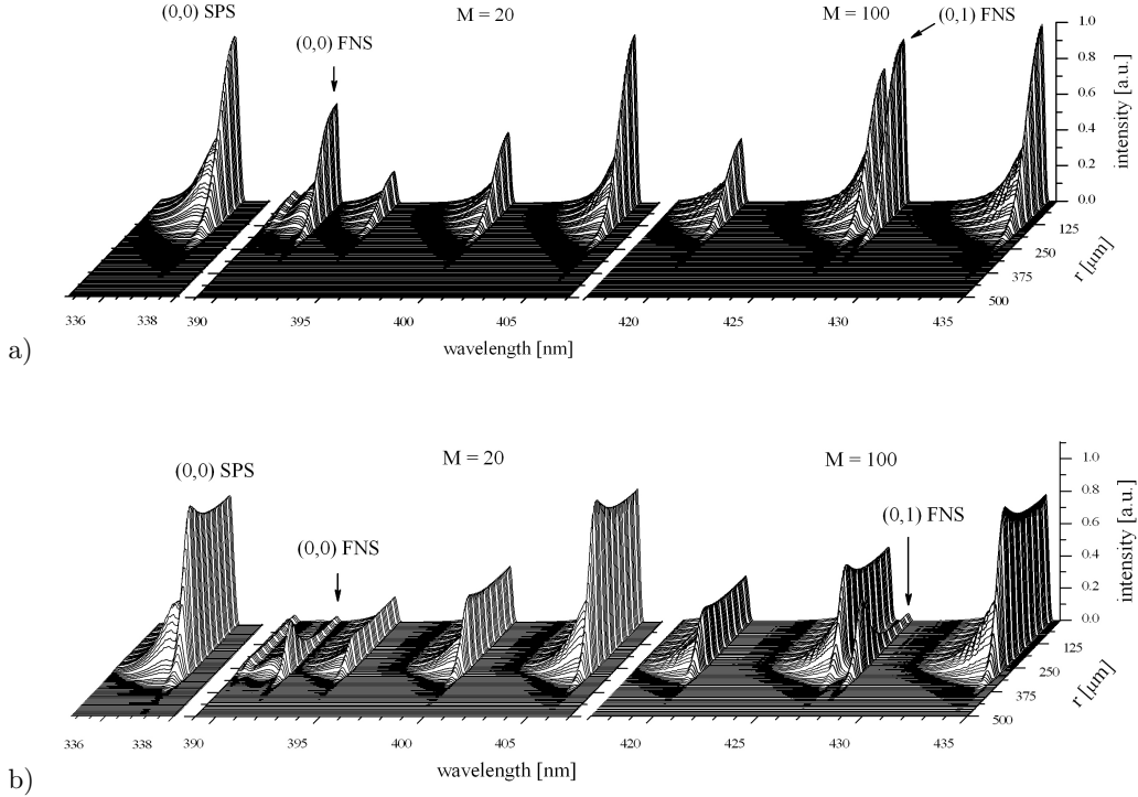
Figure 10: Synthetic streamer head emission distribution evaluated along the radius from the data shown in Fig. 6. Calculated assuming T_{rot} = 300 K and using triangular instrumental function (FWHM = 0.2 nm). Radially resolved spectra simulated at two ( x = \text{const.} ) positions corresponding to maximum axial population (indicated as FNS max in Fig.6) of the N_2^+(B^2\Sigma) state (a) and position slightly shifted ( \Delta x = 112 \mu\text{m} , i.e. approx. 200 ps delay) behind the FNS max position (b). The value M denotes the multiplication factor.
