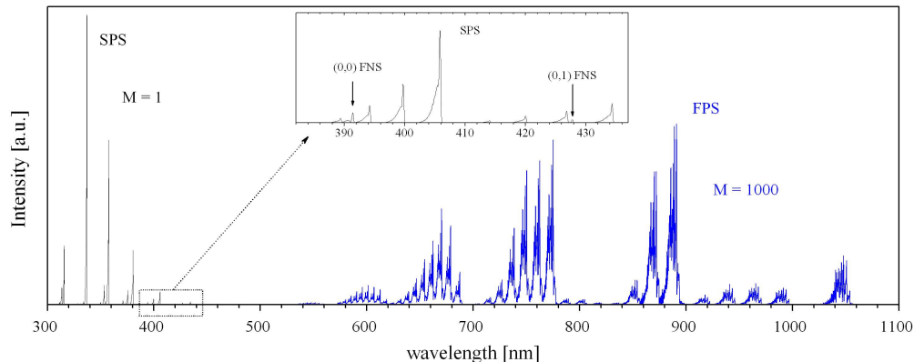
Figure 9: Synthetic streamer head emission spectrum integrated over the whole x - r plane displayed in Fig. 6. Calculated assuming T_{\text{rot}} = 300 K and using triangular instrumental function (FWHM = 0.2 nm). The value M denotes the multiplication factor.
