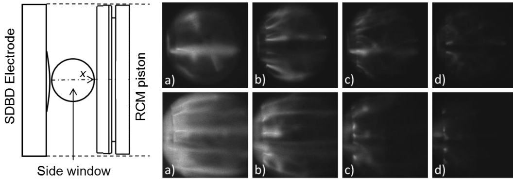
Figure 1: Side imaging of the discharge development in the RCM. n -C 7 H 16 /O 2 /N 2 mixture, T_C = 650 K. Upper row: U = 50 kV; Lower row: U = -55 kV. a) P_{TDC} = 1.5 bar b) P_{TDC} = 2.1 bar c) P_{TDC} = 2.7 bar d) P_{TDC} = 3.3 bar.
