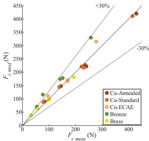
Fig. 8. Correlation between measured and predicted cutting forces.
