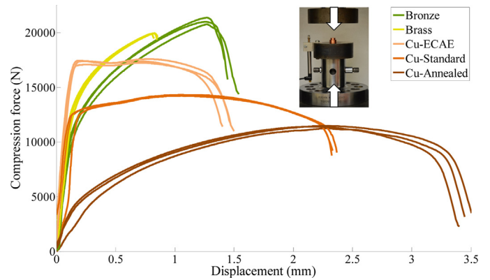
Fig. 6. Force–displacement curves of the hat-shaped shear tests.
