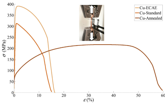
Fig. 4. Stress–strain curves of the tensile tests.
