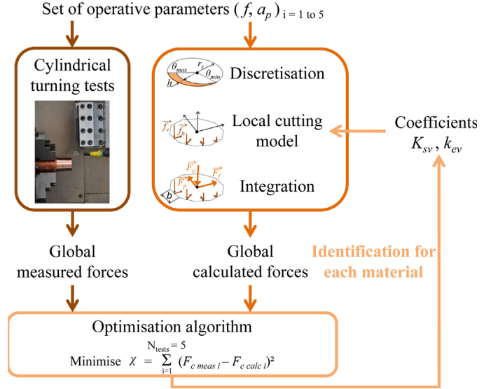
Fig. 3. Principle of the inverse identification.
