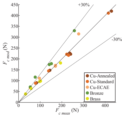
Fig. 8. Correlation between measured and predicted cutting forces.
