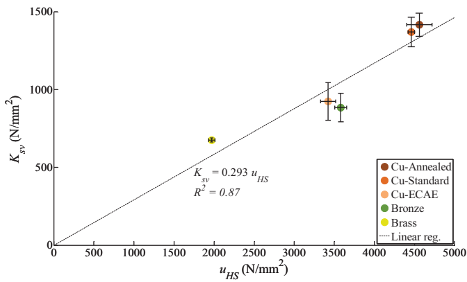
Fig. 7. Correlation between cutting coefficients and hat-shaped volumetric strain energies.
