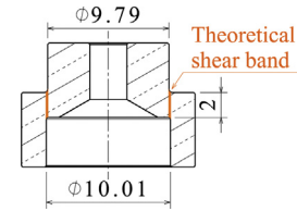
Fig. 5. Hat-shaped specimen dimensions.
