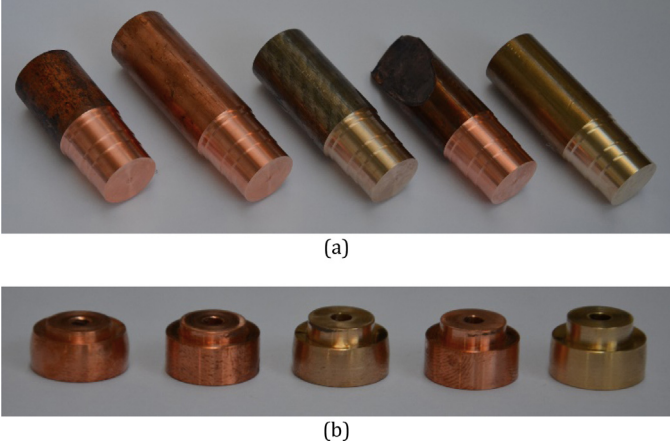
Fig. 1. The five tested materials: (a) machined samples ( \phi 35 mm); (b) hat-shaped specimens ( \phi 14 mm) after compression.
