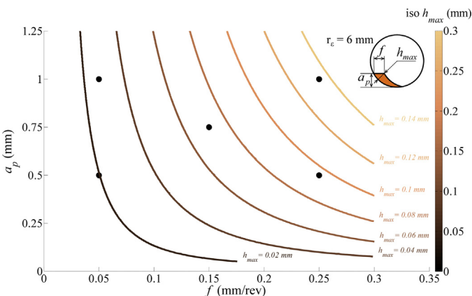
Fig. 2. Set of five cutting experiments, at constant V_c = 250 \text{ m/min} .
