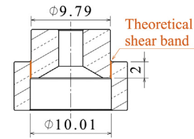
Fig. 5. Hat-shaped specimen dimensions.
