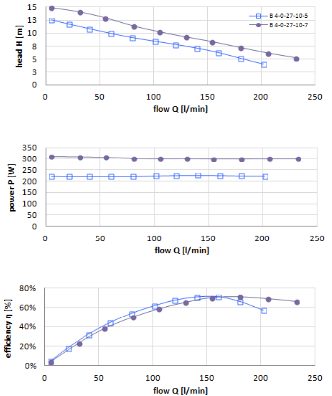
Figure 16. Head, power and efficiency over flow for outlet width 5 mm and 7 mm
