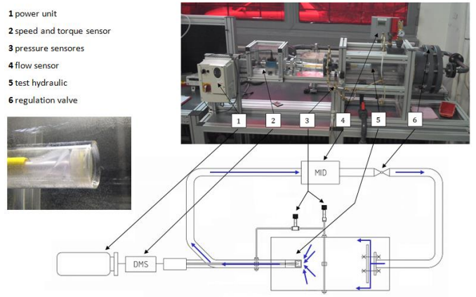
Figure 10. Test stand
