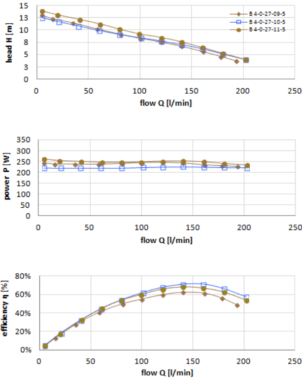
Figure 14. Head, power and efficiency over flow for d_{i1} = 9 \text{ mm}, 10 \text{ mm} and 11 \text{ mm}
