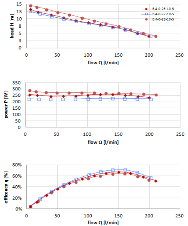
Figure 13. Head, power and efficiency over flow for d_s = 25 mm, 27 mm and 28 mm
