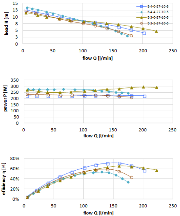
Figure 15. Head, power and efficiency over flow for blades 3 and 4 and backup-blades 3 and 4
