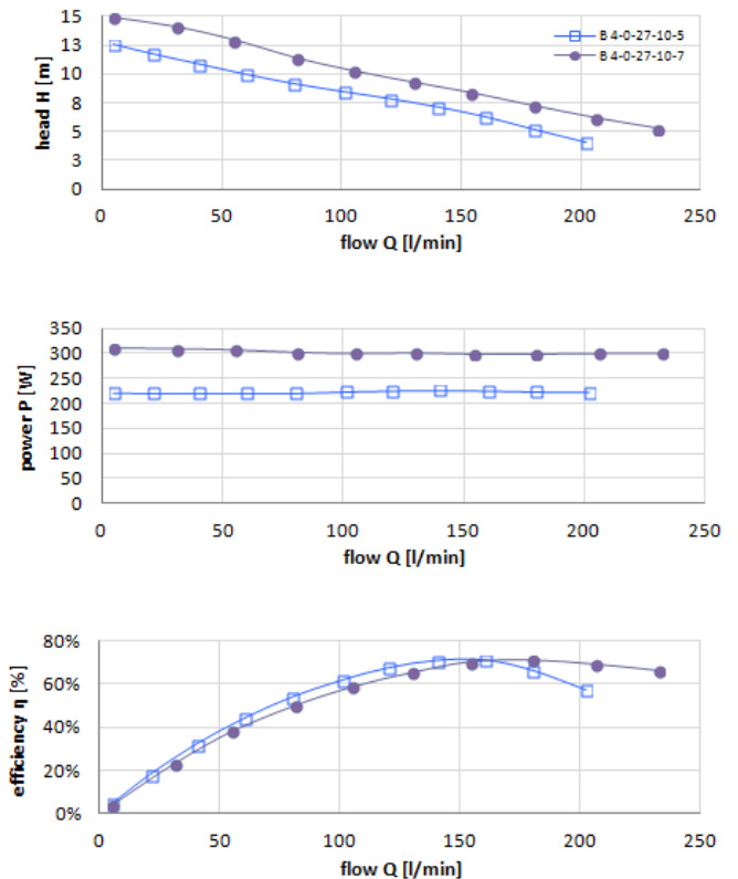
Figure 16. Head, power and efficiency over flow for outlet width 5 \text{ mm} and 7 \text{ mm}
