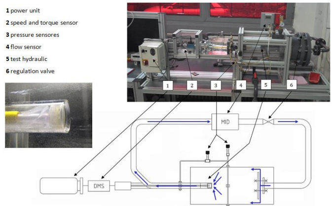
Figure 10. Test stand
