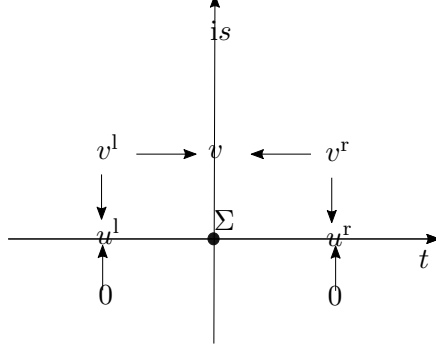
FIGURE 1. Relation between v , v^{r/l} and u^{r/l} .
