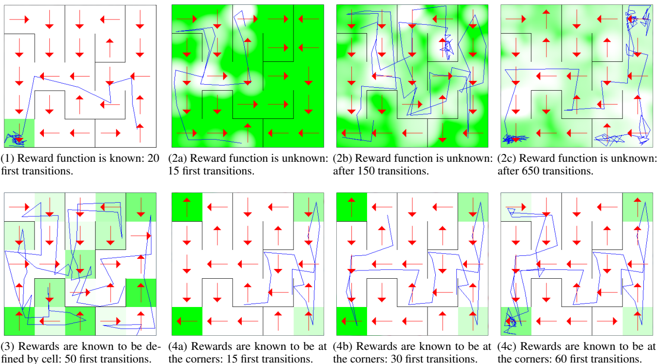
Figures 1-4: Trajectories directed by policies learnt from 25,000 transition samples with various reward function representations. Some of the policies are motivated by the knowledge of the estimated reward function and some are motivated by curiosity and optimism. The walls are displayed in black and are constant over tasks, the reward function representation are displayed in green, the current trajectory is the broken line in blue and the policy at the centre of cells is coarsely exhibited with the red arrows. In all these screenshots, the real reward function is the one rewarding the bottom left cell.
