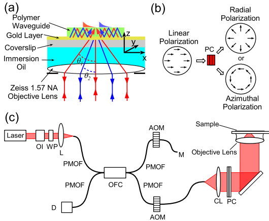
Fig. 1. Scanning surface plasmon microscope operation mode. (a) Sample configuration with the MCWG excitation through a 100\times/\text{NA } 1.57 Carl Zeiss objective lens. (b) Spatial distribution of the polarization at the entrance of the objective lens aperture. The PC switches between a radially and an azimuthally polarized beam. (c) Microscope setup including a fibered heterodyne interferometer, He Ne laser (632.8 nm); OI, optical isolator; WP, half wavelength waveplate; L, lens; PMOF, polarization maintaining optical fiber; OFC, optical fiber coupler; AOM, acousto optic modulator; D, detector; CL, collimating lens; M, mirror.
